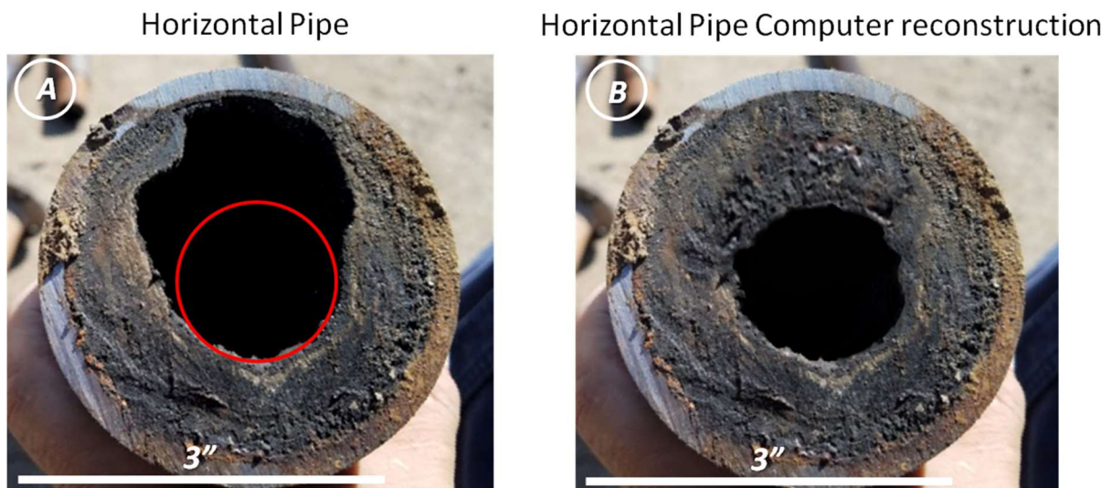
Figure 4. Asphaltene/hydrocarbon scale in the horizontal pipe after a brief HCD Multi-Flow® treatment (A) and the computer reconstruction of the asphaltene/hydrocarbon scale in the horizontal pipe before HCD Multi-Flow® treatment (B).
