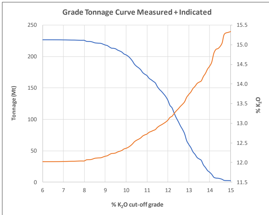
Figure 4-1: Grade-Tonnage Curve for Mineralisation that satisfies the minimum mining thickness
