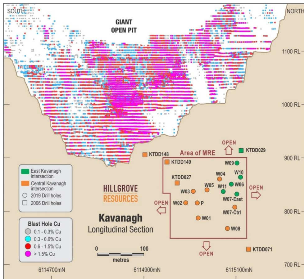
Figure 2 Longitudinal section of the drill holes and the extent of the MRE
