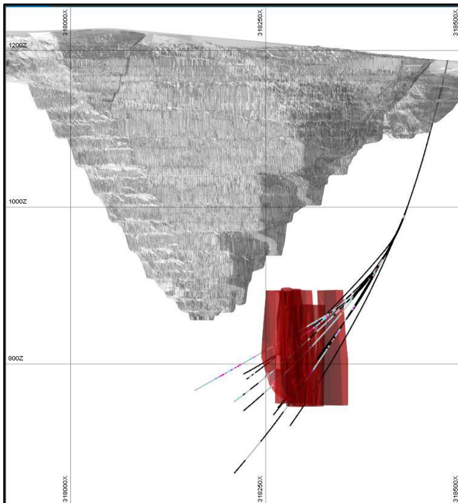
Figure 1 Location of 2019 Mineral Resource Estimate and 2019 drill holes
