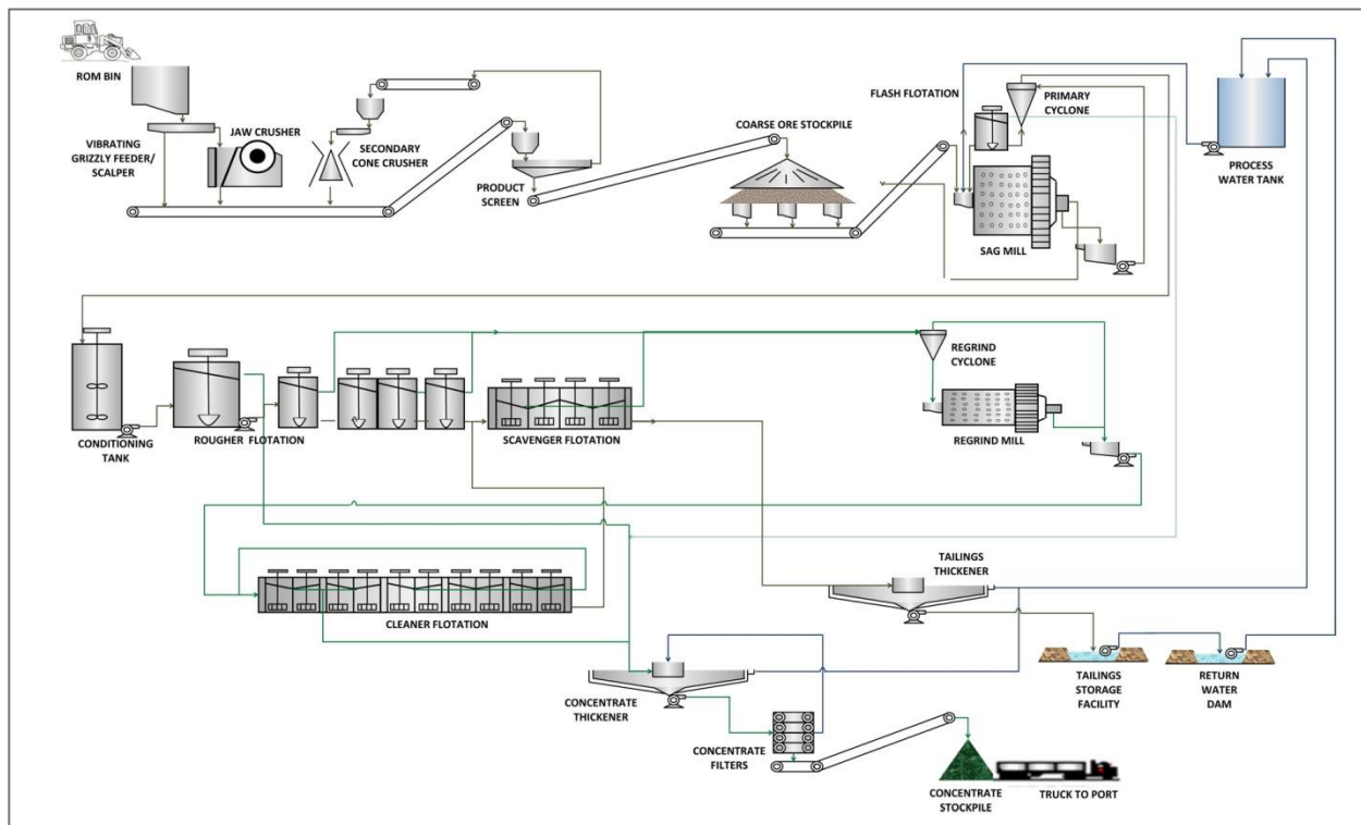
Figure 39: Kanmantoo processing plant simplified flowsheet
