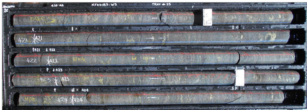
Figure 4: Central Kavanagh core (KTDD187_W5 from 420m to 424.7m downhole) showing mineralised BCGS
