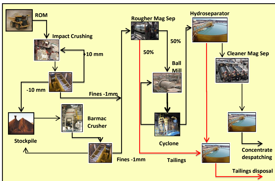
Figure 1. Simplified process flow sheet, Hawsons Iron Project
