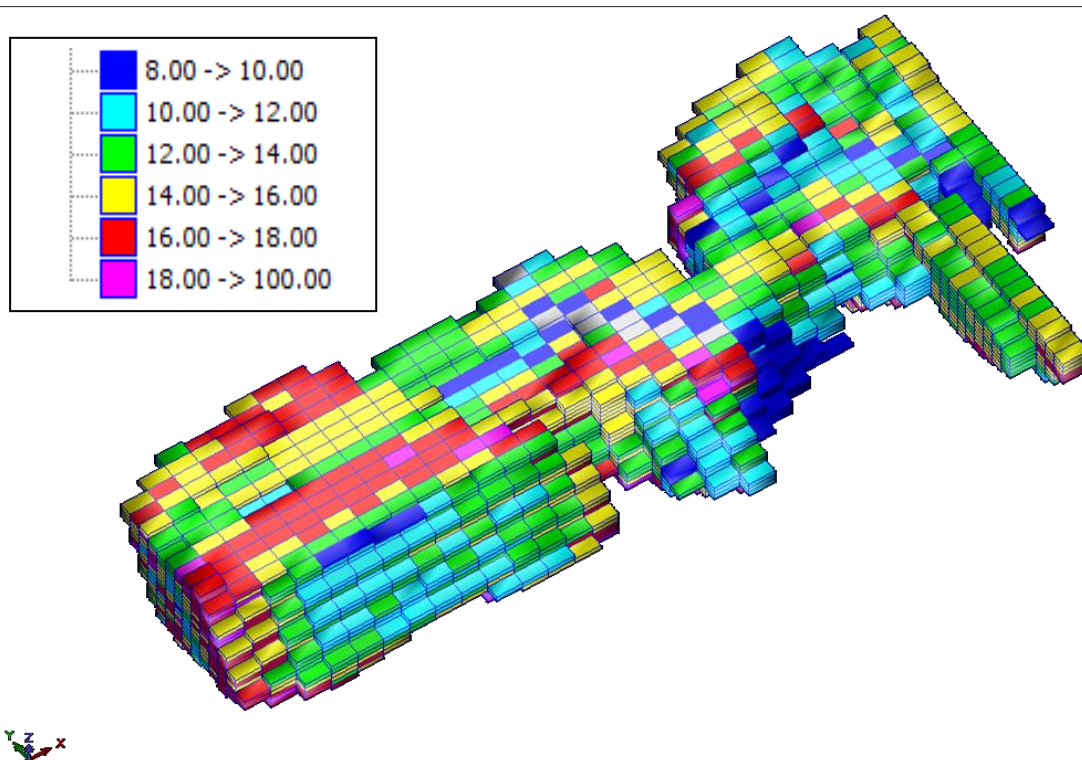
Figure 10 Block Model DTR Magnetite Grade Distribution for Main Magnetite Zone
