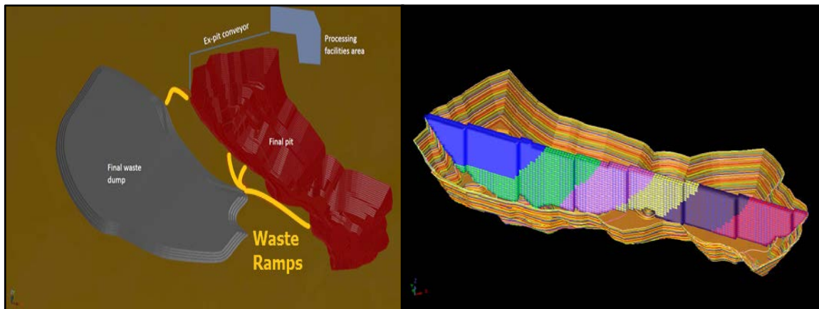
Mine layout and pit cross section
