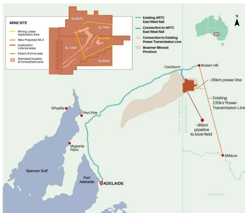
Hawsons Iron Project and Tenement Map
