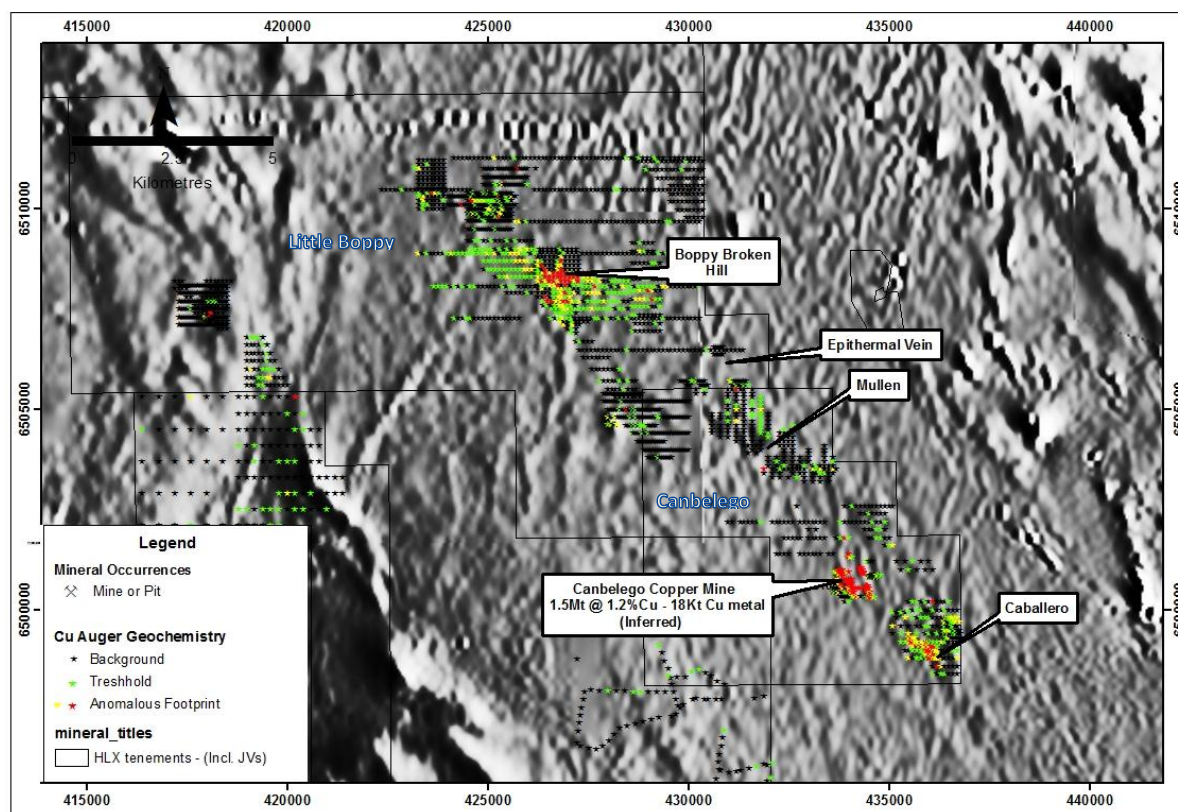
Figure 2: Copper in soil geochemistry in Canbelego JV & Little Boppy 100% Oxley area. Priority EM and Drilling targets for 2H 2012.
