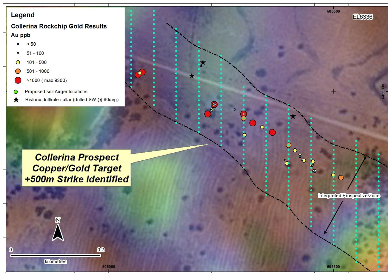
Figure 4: Proposed Auger soil program over Gold rockchip results on magnetics and aerial photo
