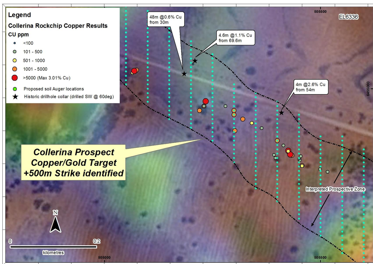
Figure 3: Proposed Auger soil program over Copper rockchip results on magnetics and aerial photo
