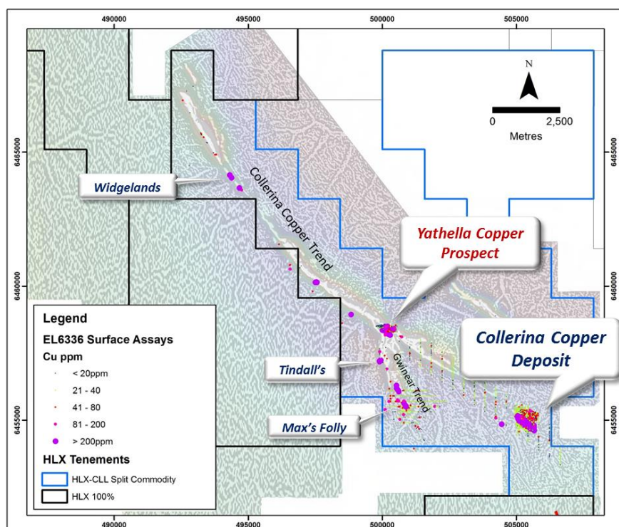
Figure 3: Yathella Copper Prospect, located on the Collierina Copper Trend 6km NW from the Collierina Copper Deposit
