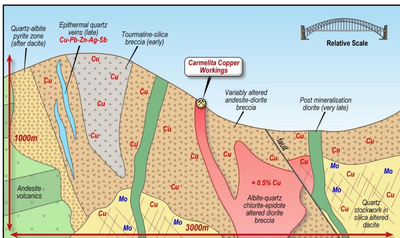
Figure 2 | Joshua Porphyry System - Interpreted schematic E-W geological model in E-W section.
