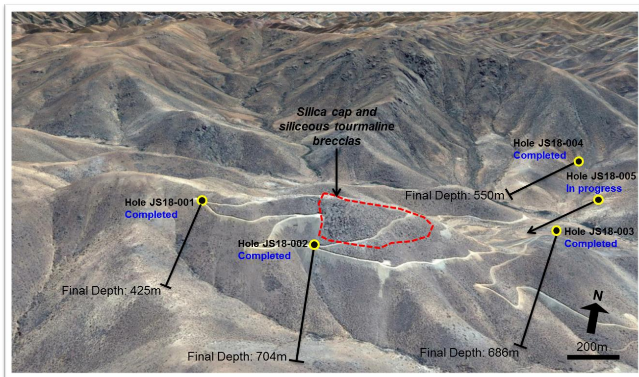
Figure 1 | Relative positions of 2018 drill holes at Joshua shown on north-looking Google image.
