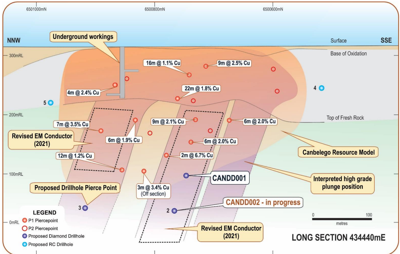
Figure 2: Schematic long section of Canbelego Copper deposit 2 with re-processed DHEM conductor target and approximate location of drill hole pierce points for CAND001 (complete) and CAND002 (In progress)
