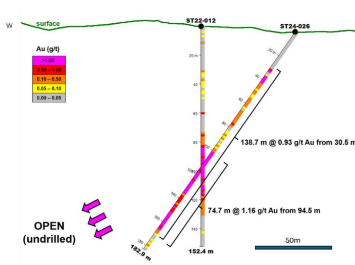
Figure 8: Stealth cross section of drillholes 012 and 026 coloured by gold grade and showing wide zones of oxide gold mineralisation open to W. Multiple 0.25 to 0.50 mm occurrences of visible gold were identified in RC chip trays indicating a potential plunge zone to the west.
