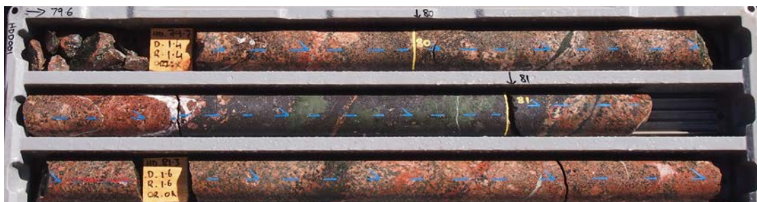
Semi-massive magnetite-actinote-chlorite-hematite alteration is a common component of the Dronfield western anomaly system (HDD001, 81m)
