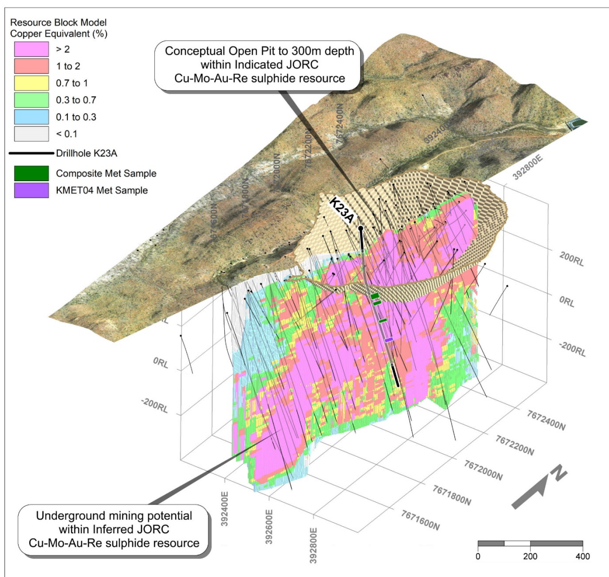
Figure 2. Oblique view of the Kalman Deposit showing the location of K-23A utilised in the ore sorting trial
