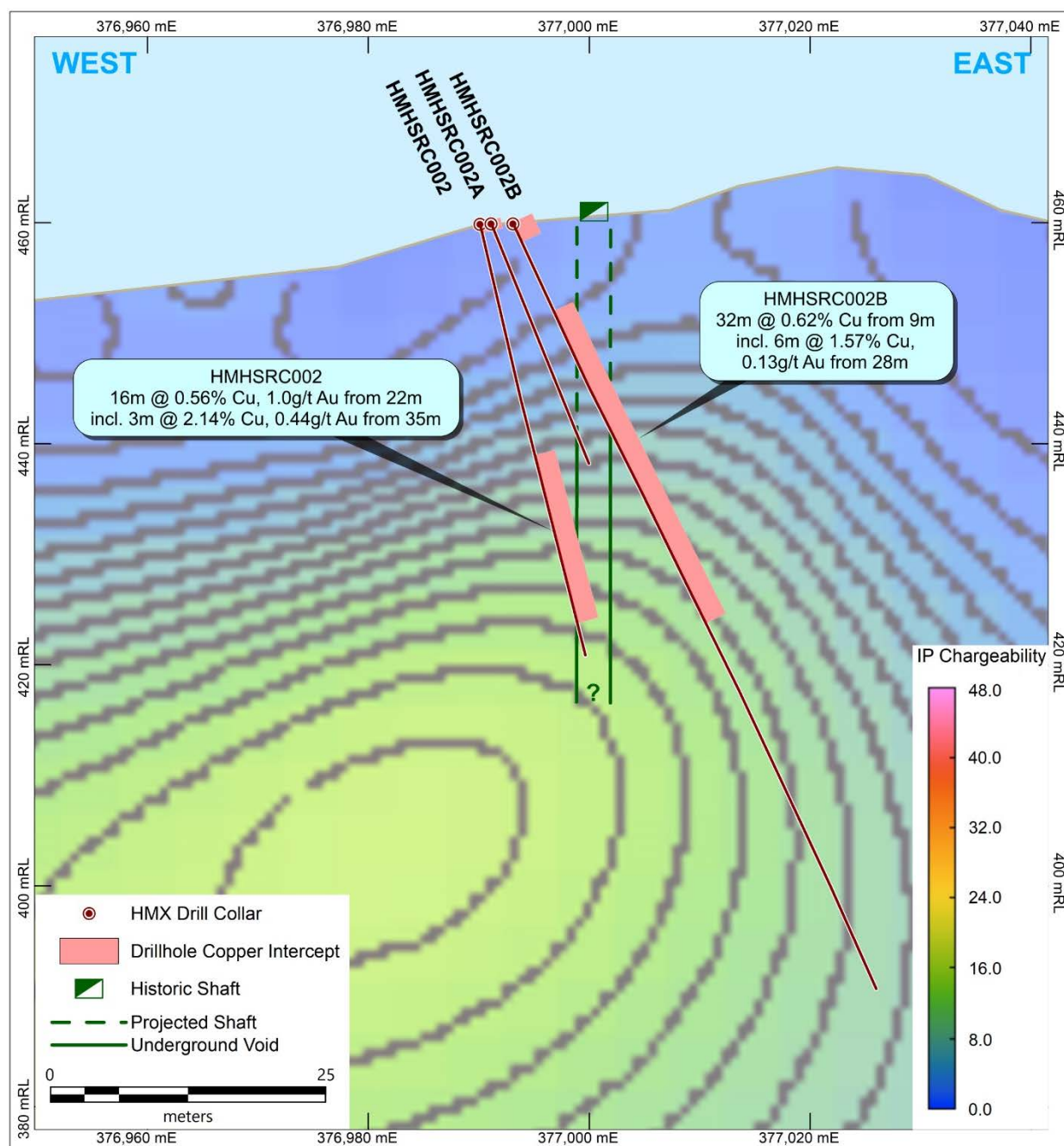
Figure 9. Cross section 7658435mN (The Stubby prospect), looking north. Back drop is IP chargeability.
