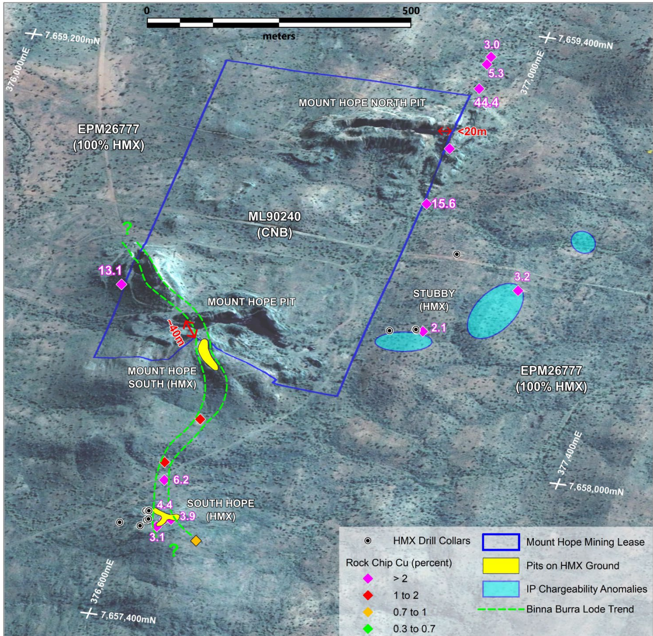
Figure 8. Mount Hope Plan showing recently completed drill-holes and the chargeability response from the IP survey lines. See ASX Announcement 22 November 2022 and 4 July 2023.
