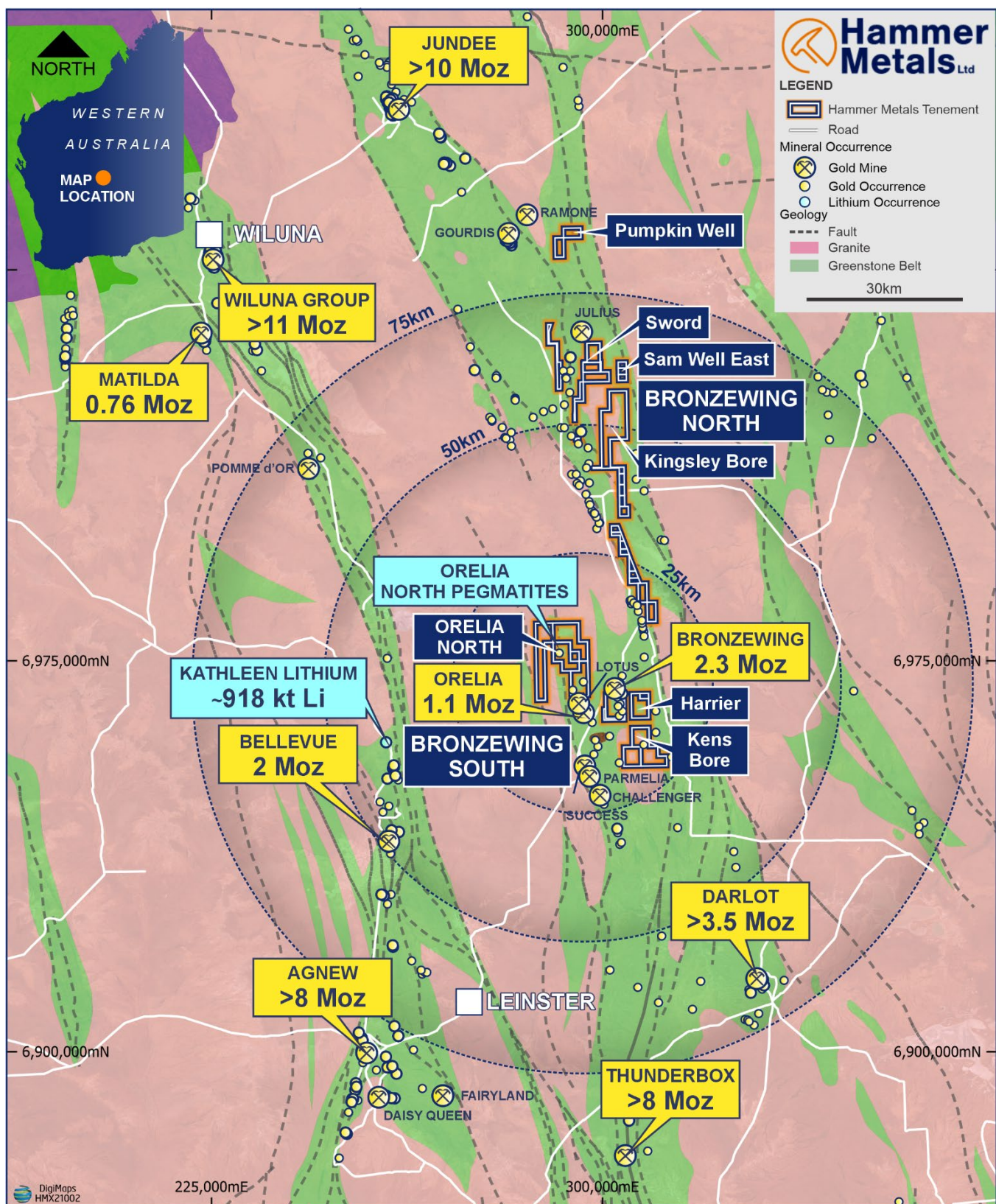
Figure 15. Hammer Metals Yandal Project tenements, showing the location of the Sword and Harrier Prospects
