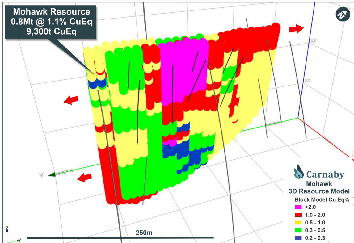
Figure 13. Mohawk MRE coloured by block model centroid CuEq% grades.
