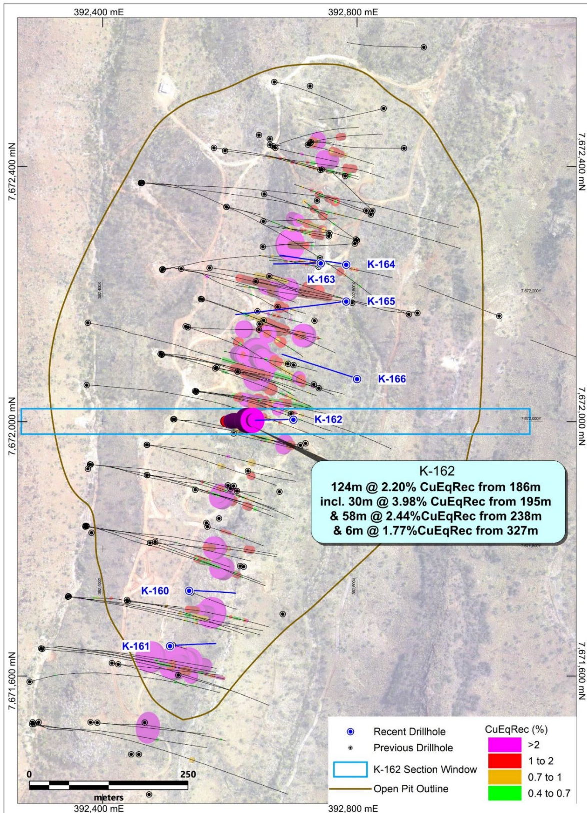
Figure 3. Kalman Deposit plan view showing historic drilling and the location of holes in the current program. The brown line represents the outline of a conceptual pit to ~370m depth. Refer to ASX announcement dated 8 May 2023 for background on all historic drilling at Kalman.
