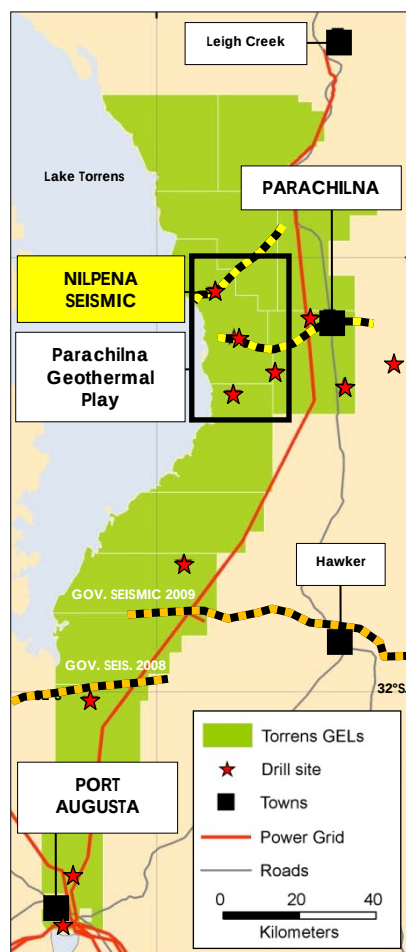
Parachilna Geothermal Play location diagram, South Australia.
