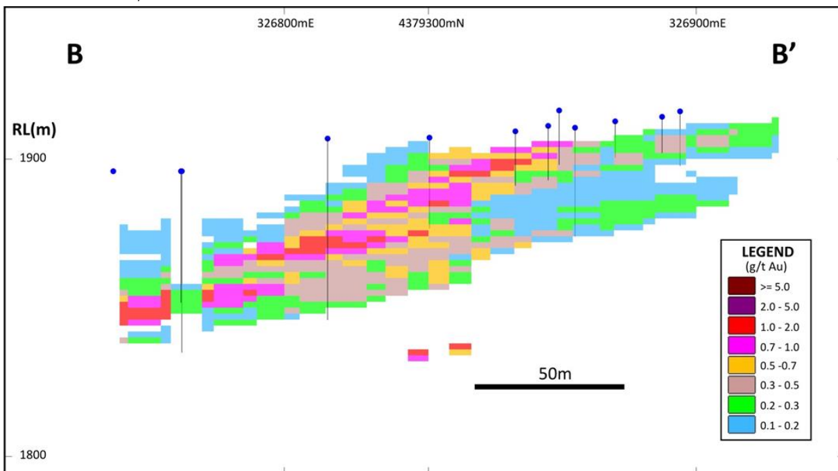
Figure 8: Mizpah cross section B-B' suggests that the mineralisation is stratigraphic, dipping at approximately 20° to the west and open down dip to the west. A second deeper horizon is present.
