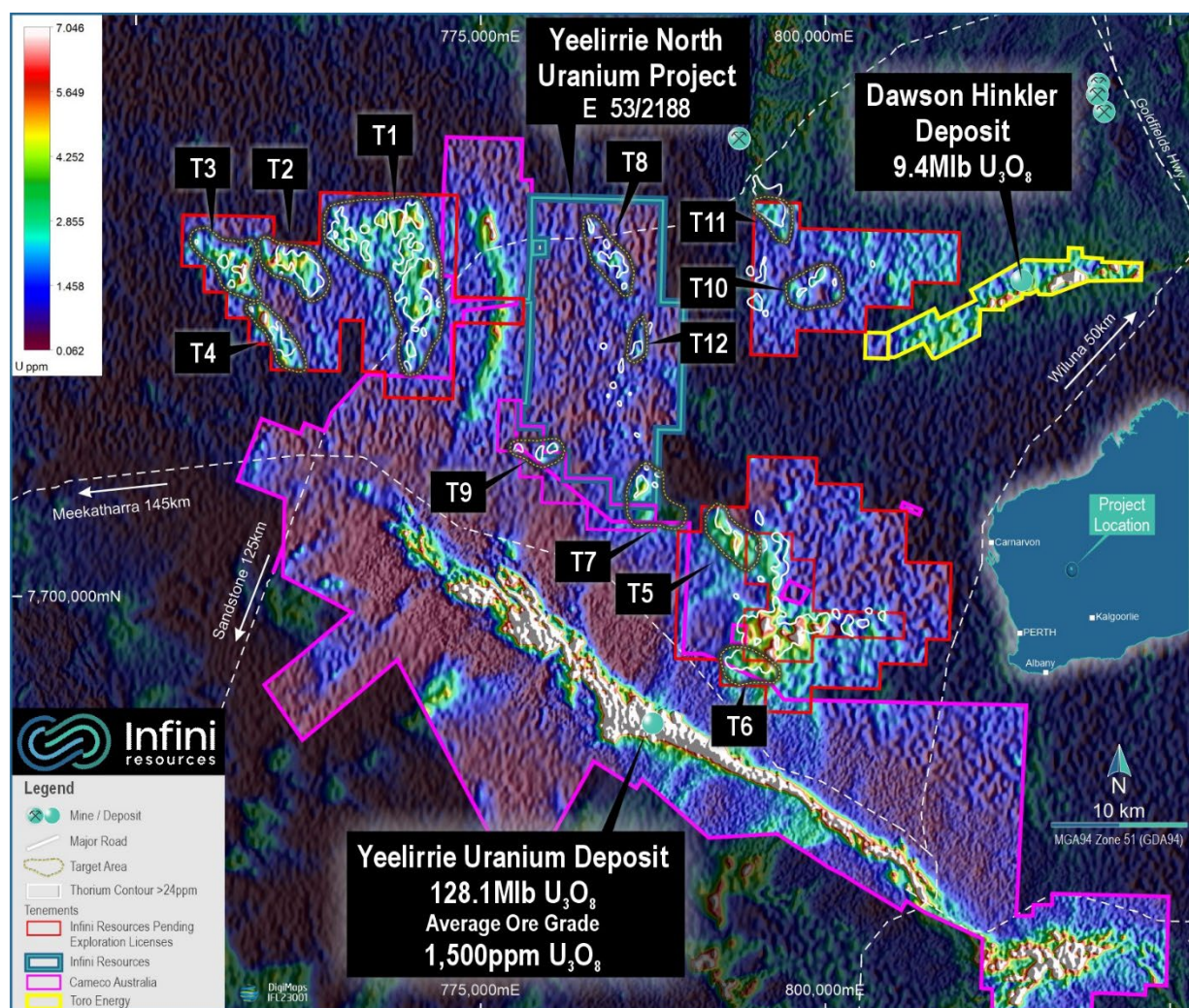
Figure 1 Location of the newly staked exploration licenses (highlighted red) at the world-class Yeelirrie uranium camp showing the geological rationale with extensive and coincidental uranium-thorium anomalism identified in regional radiometrics.
