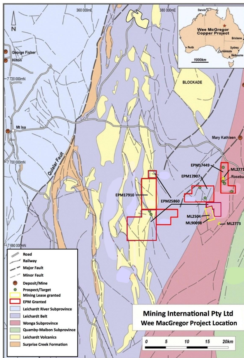
Figure 4: Wee MacGregor Project Location and Geology
