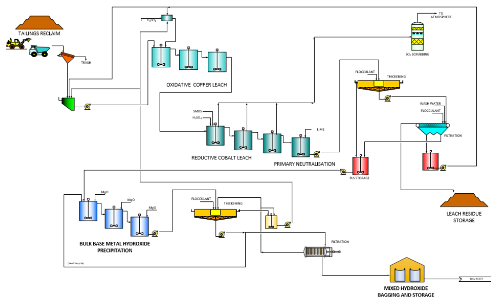
Figure 2: Kipushi Process Flowsheet
