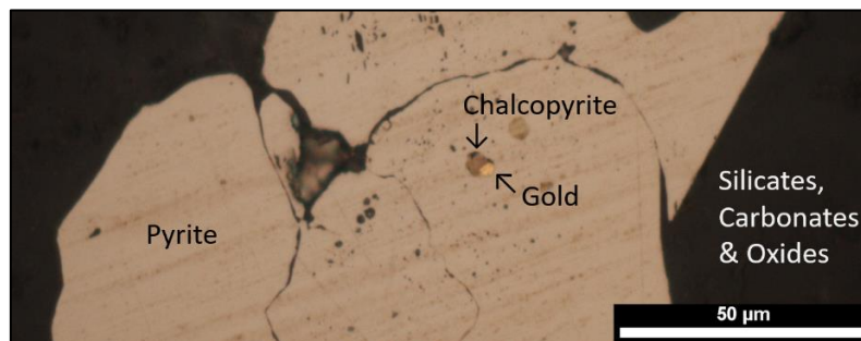
Figure 22: Photomicrograph of gold observed at 224.6m in FMDD0032 at the Everleigh target area.
