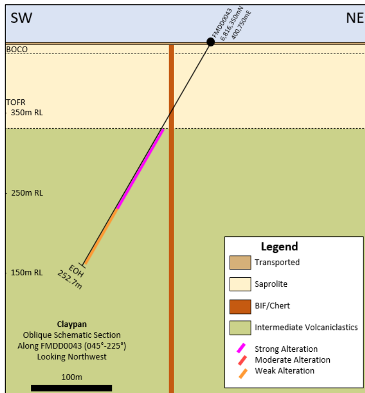
Figure 11: Oblique schematic section along the trace of hole FMDD0043, looking northwest. The strong alteration zone is located to the west of the BIF/SCT.
