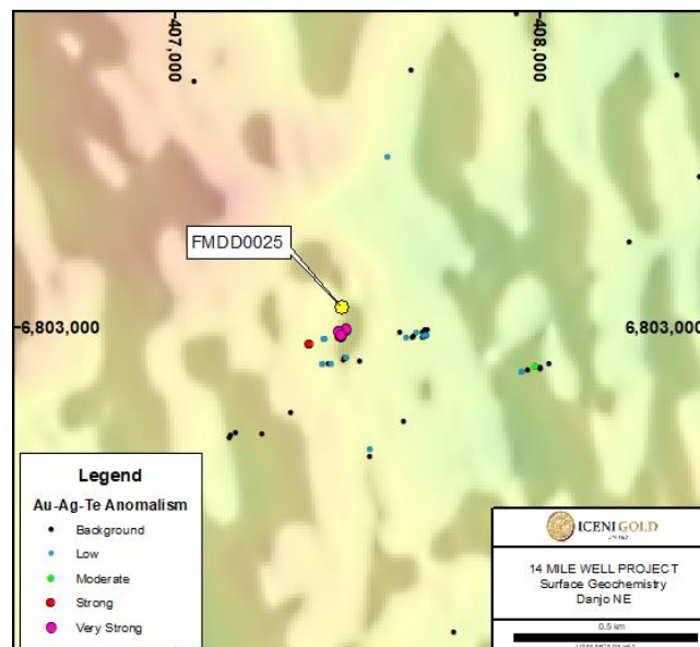
Figure 28: Danjo NE: Geochemistry illustrating the combined anomalism for Au, Ag and Te in surface rockchip sampling. The first DD hole FMDD0025, tested beneath the zone of strongest anomalism at Danjo NE. Background image is TMI RTP magnetics.
