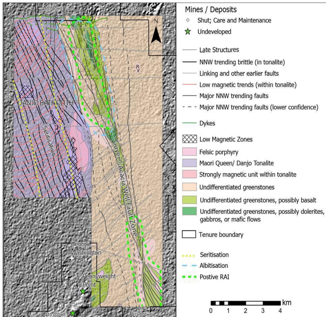
Figure 15: Interpreted geology and alteration zones within the Guyer Well target area. The main structural corridor has a length of 15km within the 14 Mile Well project area.
