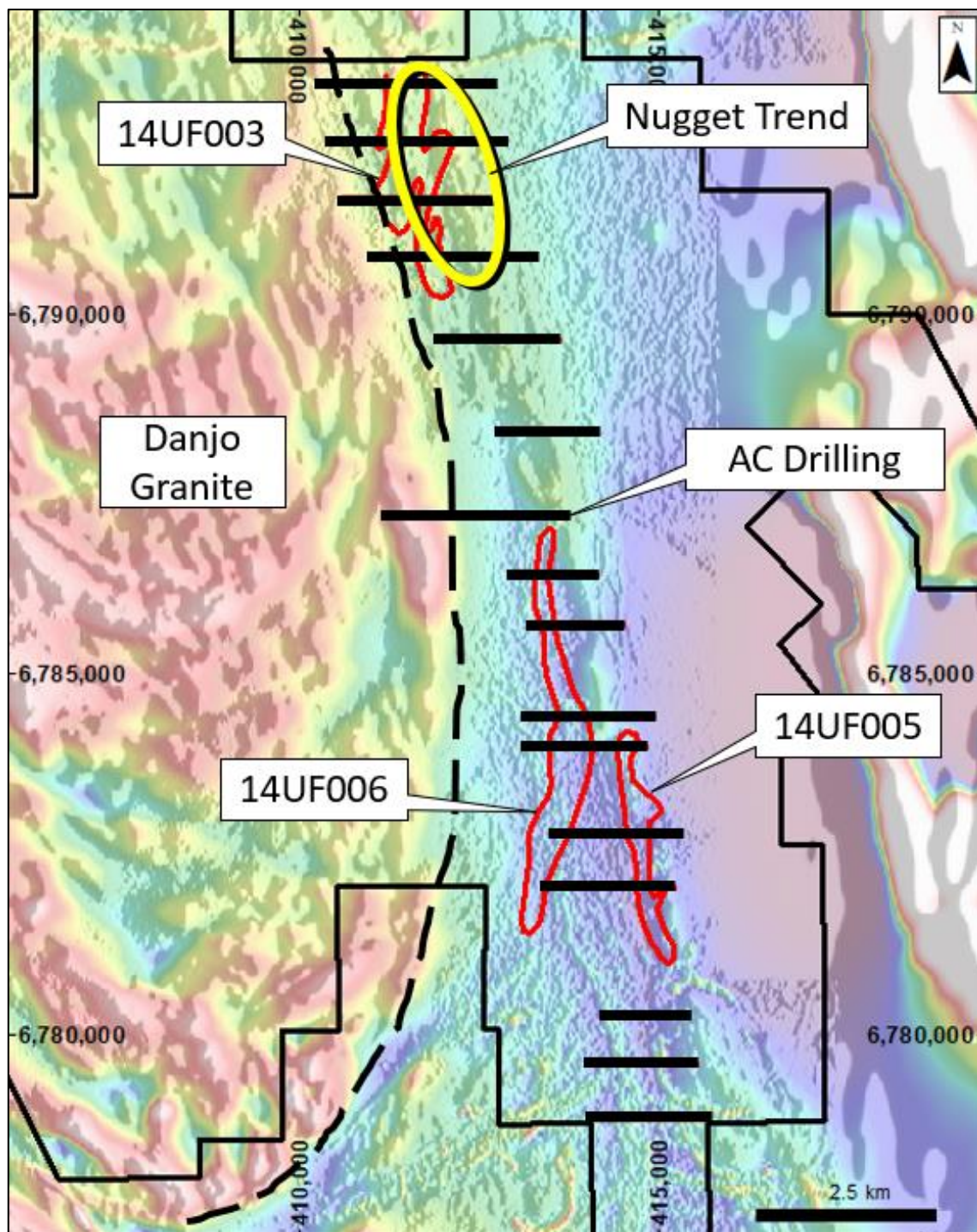
Figure 5: Plan showing the location of the Air Core drilling relative to the UFF+ anomalies and the gold nugget trend within the Guyer target area. Background image is magnetics TMI RTP.
