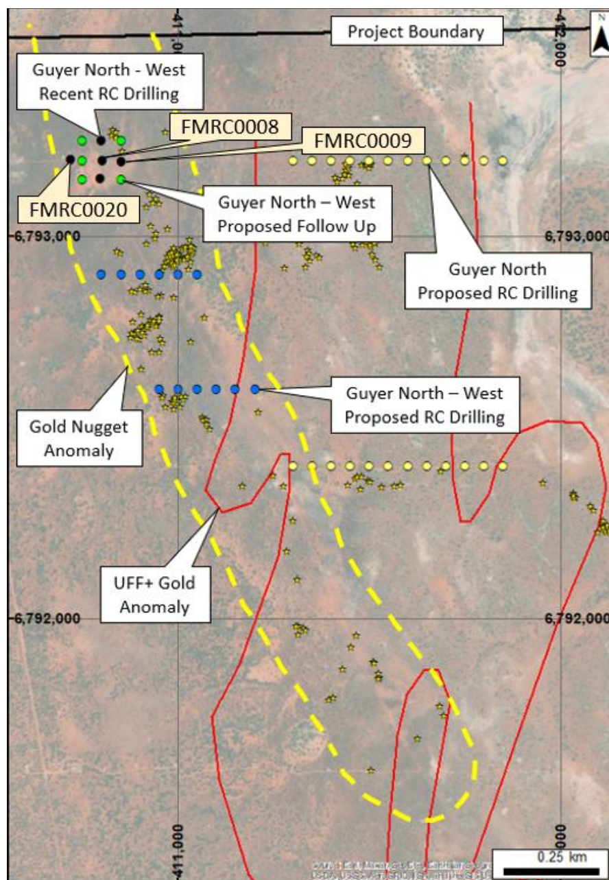
Figure 2: Collar Plan showing the location of recent drilling relative to surface gold anomalism.
