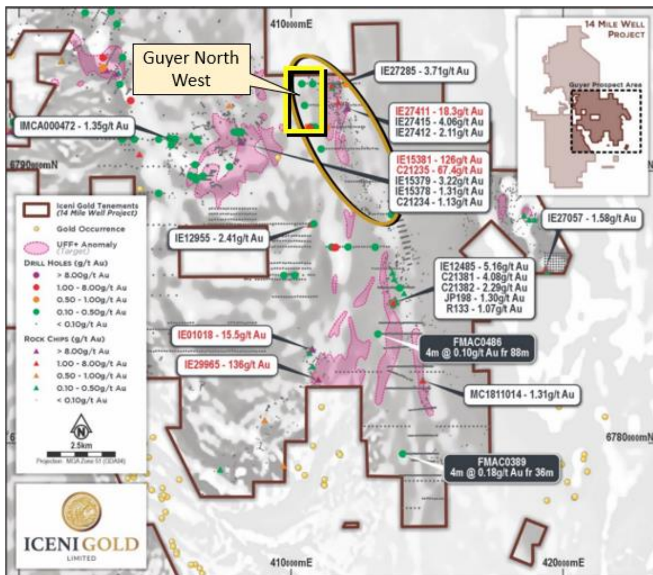
Figure 6 Gold anomalism in the Guyer Trend and the location of Guyer North - West (ASX release 20 July 2023).
