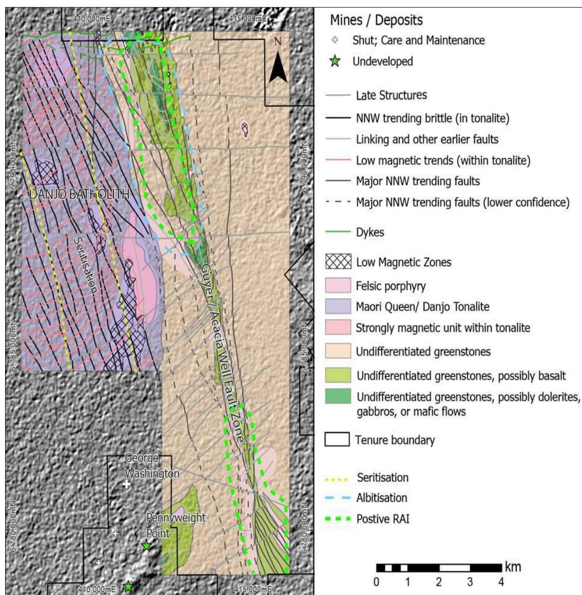
Figure 5 Interpreted geology and alteration zones of the Guyer Well Target Area (Icení prospectus 3 March 2021).
