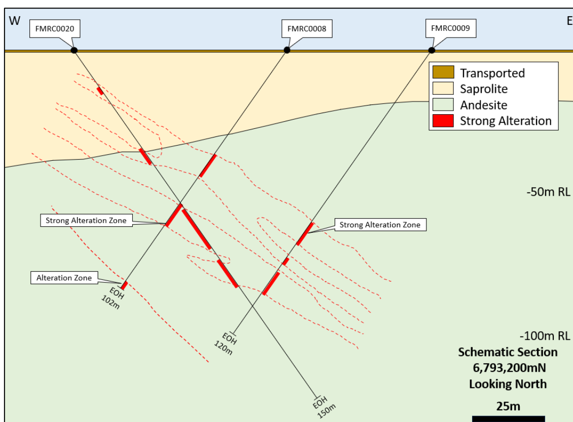
Figure 3: Section 6,793,200mN at Guyer North – West showing mineralised intervals intersected in adjacent holes.
