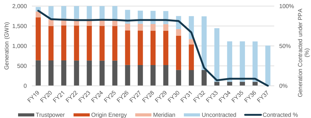
Figure 9: Forecast Generation Volume (GWh) – Operating Assets
