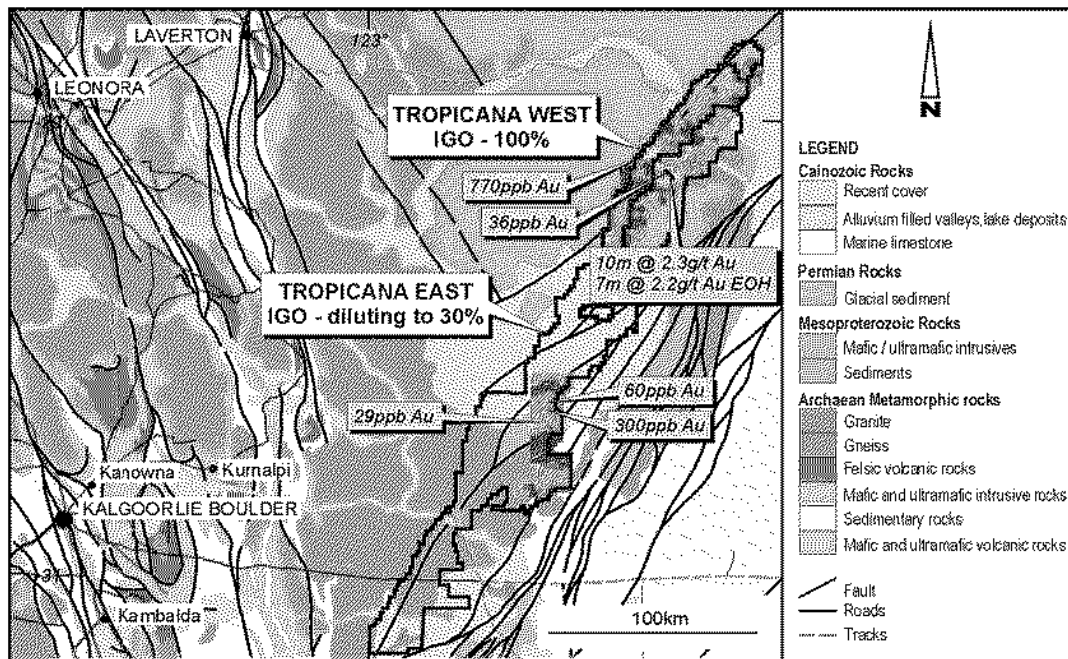
Figure 8: Tropicana – Regional Location and Gold Geochemical Anomalies
