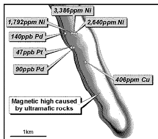
7(b):Duketon JV – Peak Soil Values Over Magnetics
