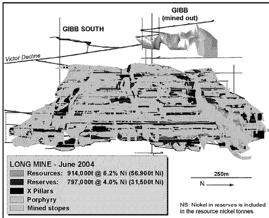
Figure 1: Long – Resource and Reserves
