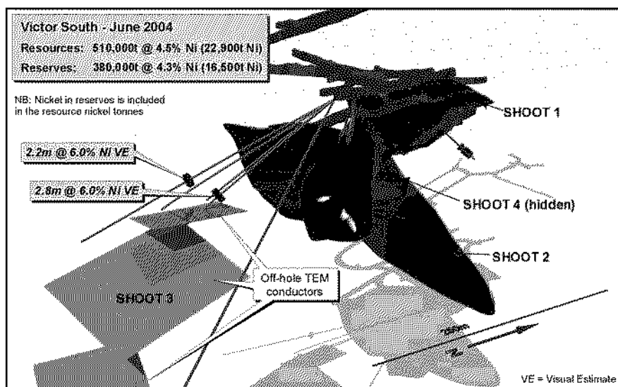
Figure 2: Victor South – 3-dimensional Model
