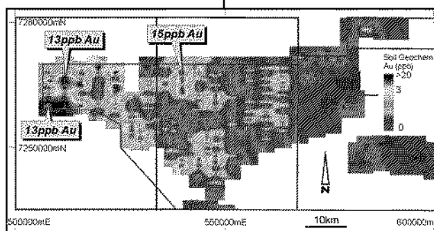
Figure 10: Musgrave Joint Venture – Bloods Range Project Gold Soil Geochemistry
