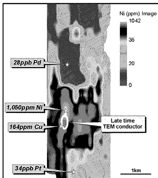
Figure 6(a): Cullen JV – Soils Peak Values Over Image of Ni Soil Geochemistry
