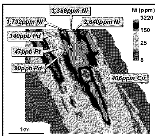
Figure 7(a): Duketon JV – Soils Peak Values Over Image of Ni Soil Geochemistry
