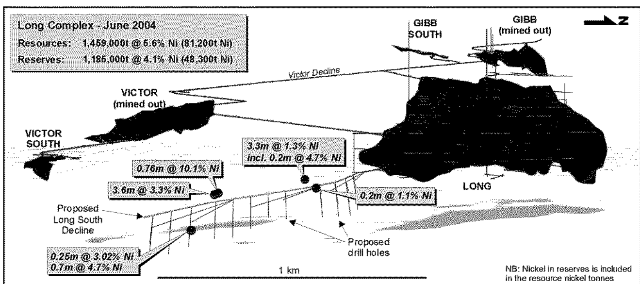
Figure 4: Long Nickel Mine – Resources, Reserves and Location of Proposed Long South Decline
