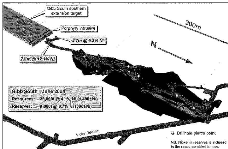
Figure 3: Gibb South – 3-dimensional Model
