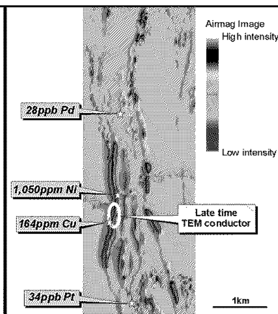
Figure 6(b): Cullen JV – EM Conductor Over Magnetics
