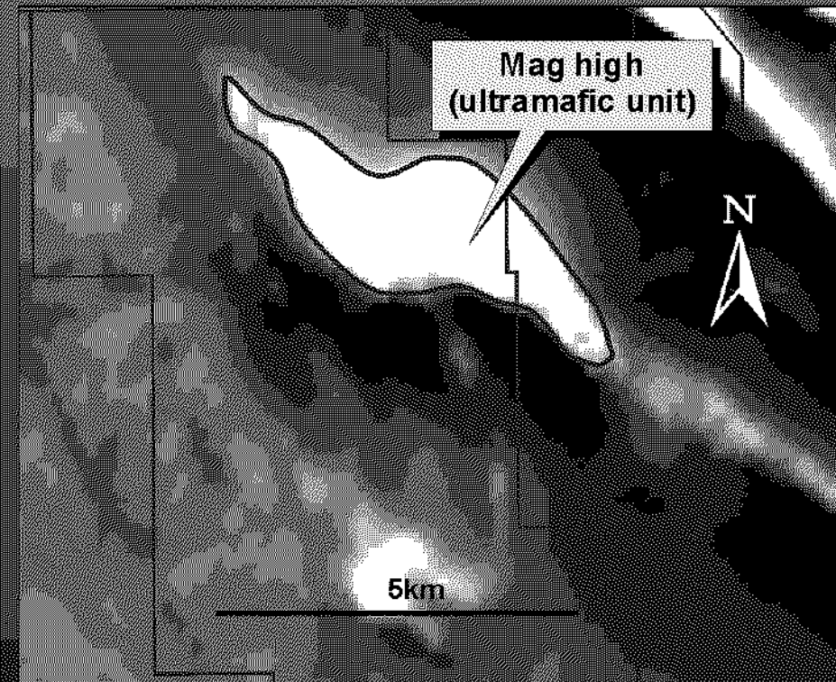
Aeromagnetic image
