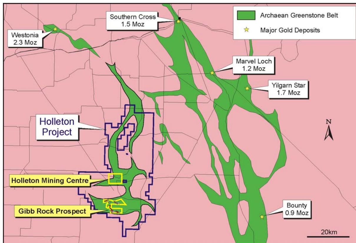
Figure 15: Holleton Project – Project Tenure Over Regional Geology Showing Historic Au Geochemical Coverage and Large Gold Mines in the District
