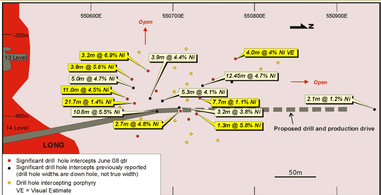
Figure 2: Long Nickel Mine – 07 Shoot Longitudinal Section Showing Drill Drive Proposed Extension and Recent Drill Intercepts
