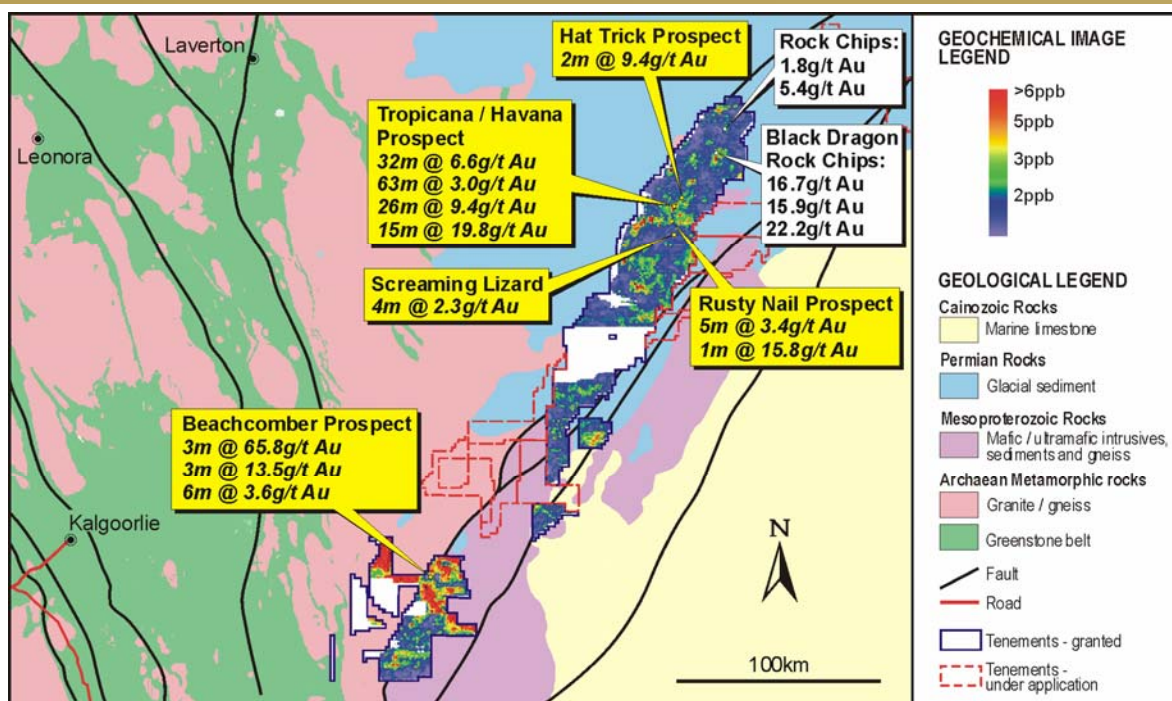
Figure 9: Tropicana JV – Significant Regional Drill-hole, Rock Chip and Geochemical Gold Anomalies in Relation to Tropicana/Havana Prospects
