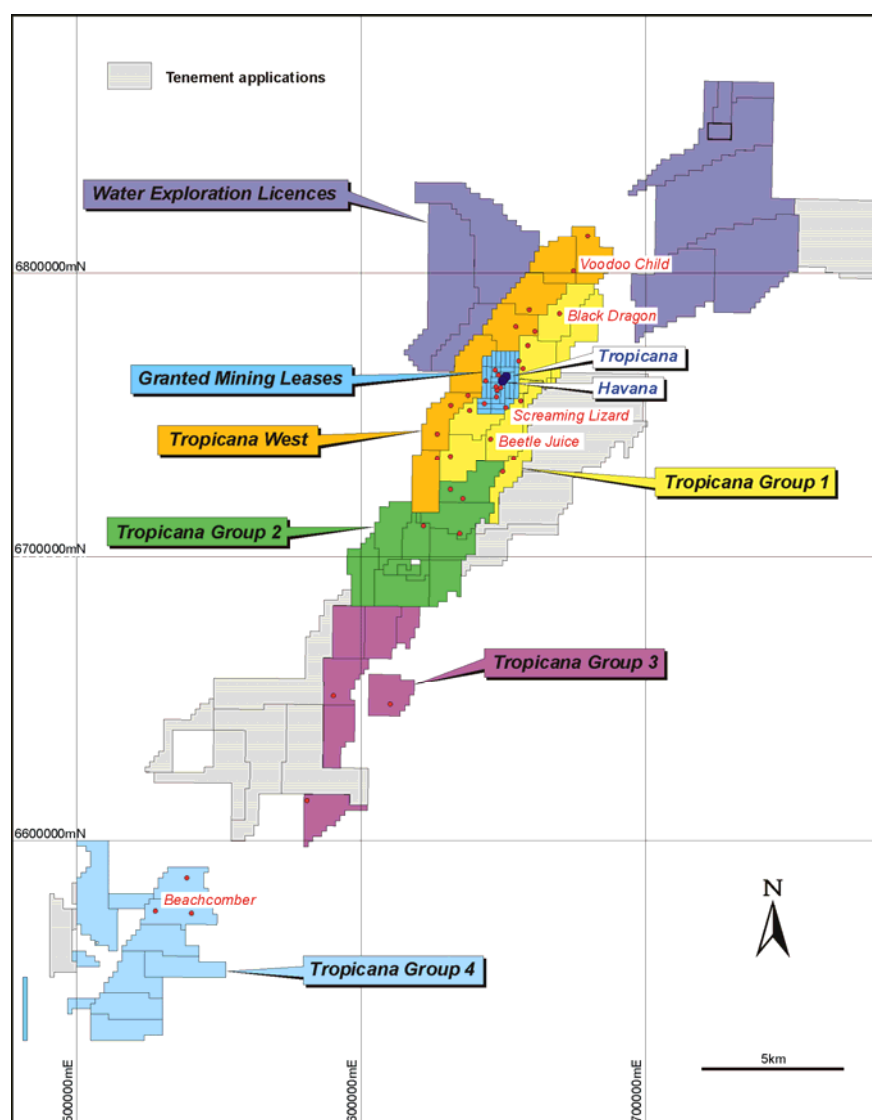
Figure 10: Tropicana JV – Tenement Groups and Prospect Locations
