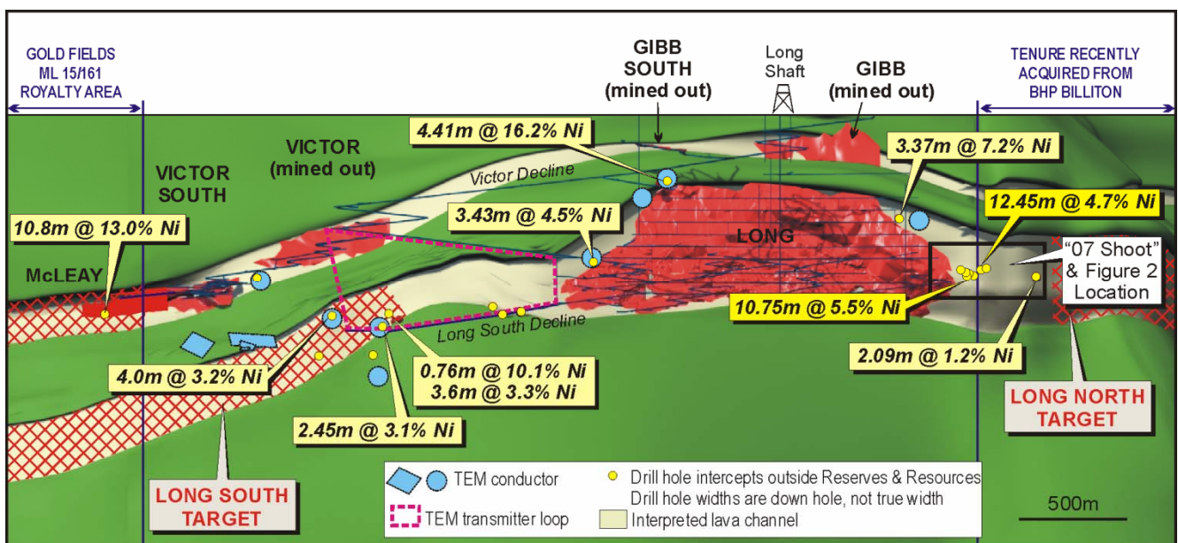
Figure 1: Long Nickel Mine – Longitudinal Section Showing New 07 Shoot, TEM Anomaly (Detail Figure 2), Long South TEM Anomaly Location, Lava Channels, and Significant Intercepts Outside Current Resources
