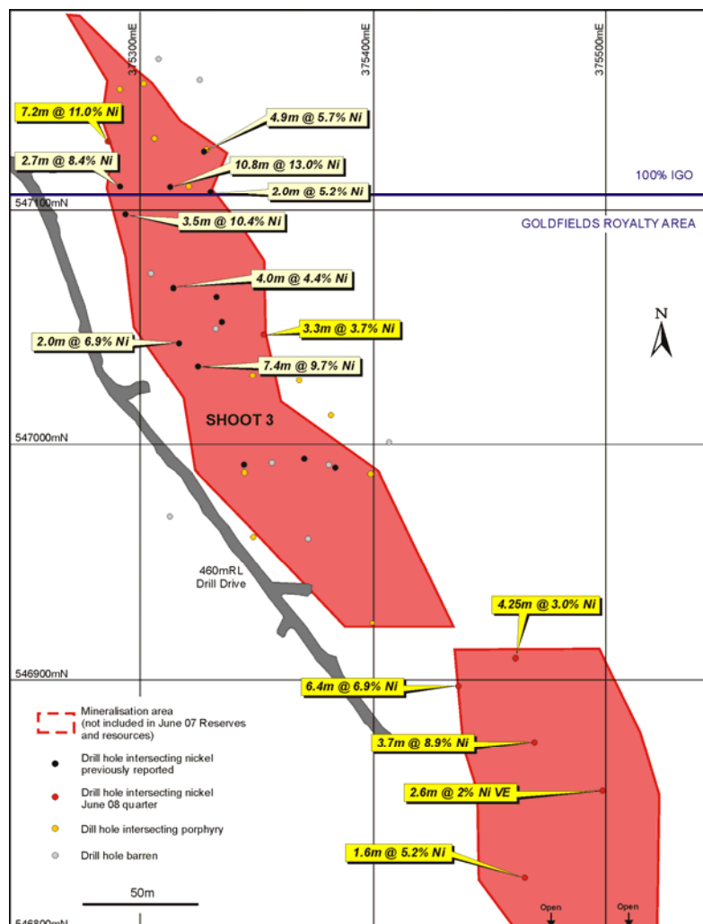
Figure 4: McLeay – Shoot 3 Plan Showing 460 Drill Drive and Recent Drill Intercepts
