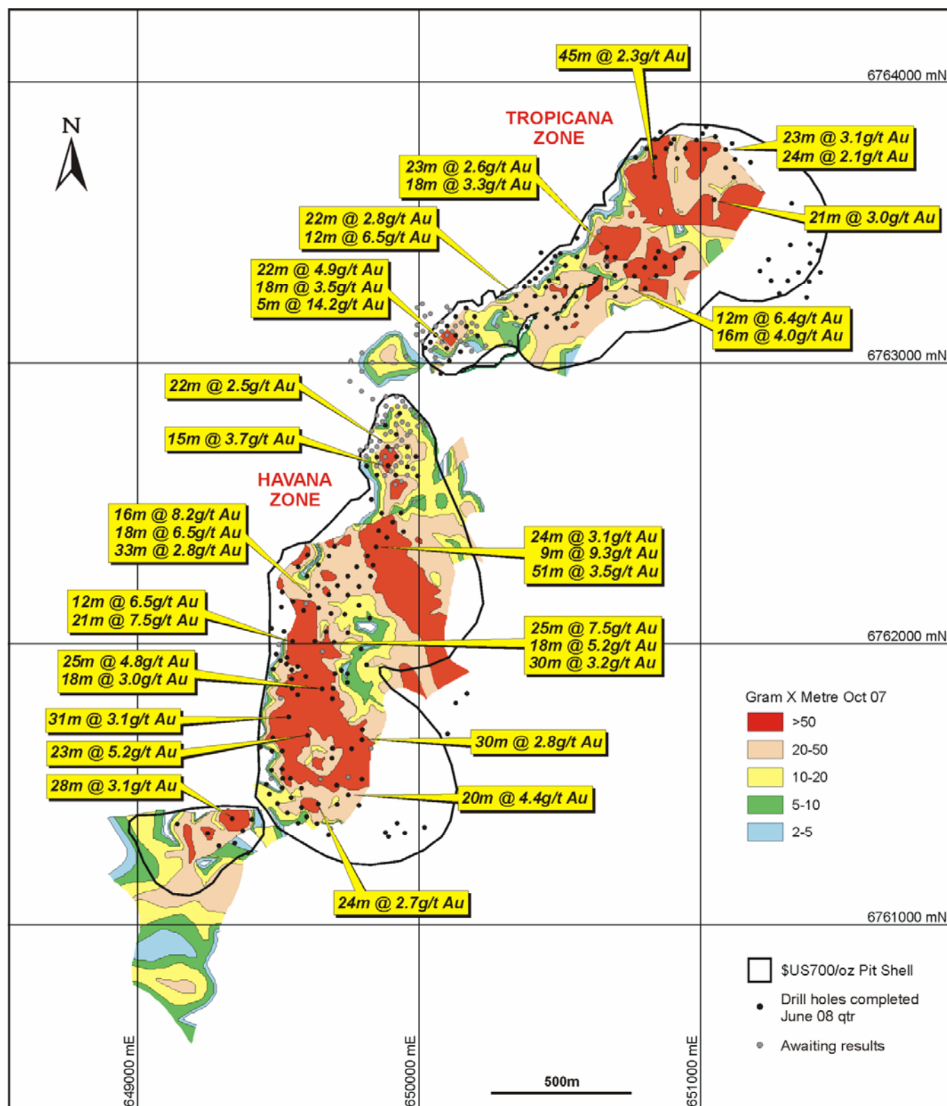
Figure 8: Tropicana JV – Prospect Plan Showing Significant Intercepts Within November 2007 Resource Outline, g/t Au x Thickness Contours and Location of Havana and Tropicana Open Pit Resource Outlines
