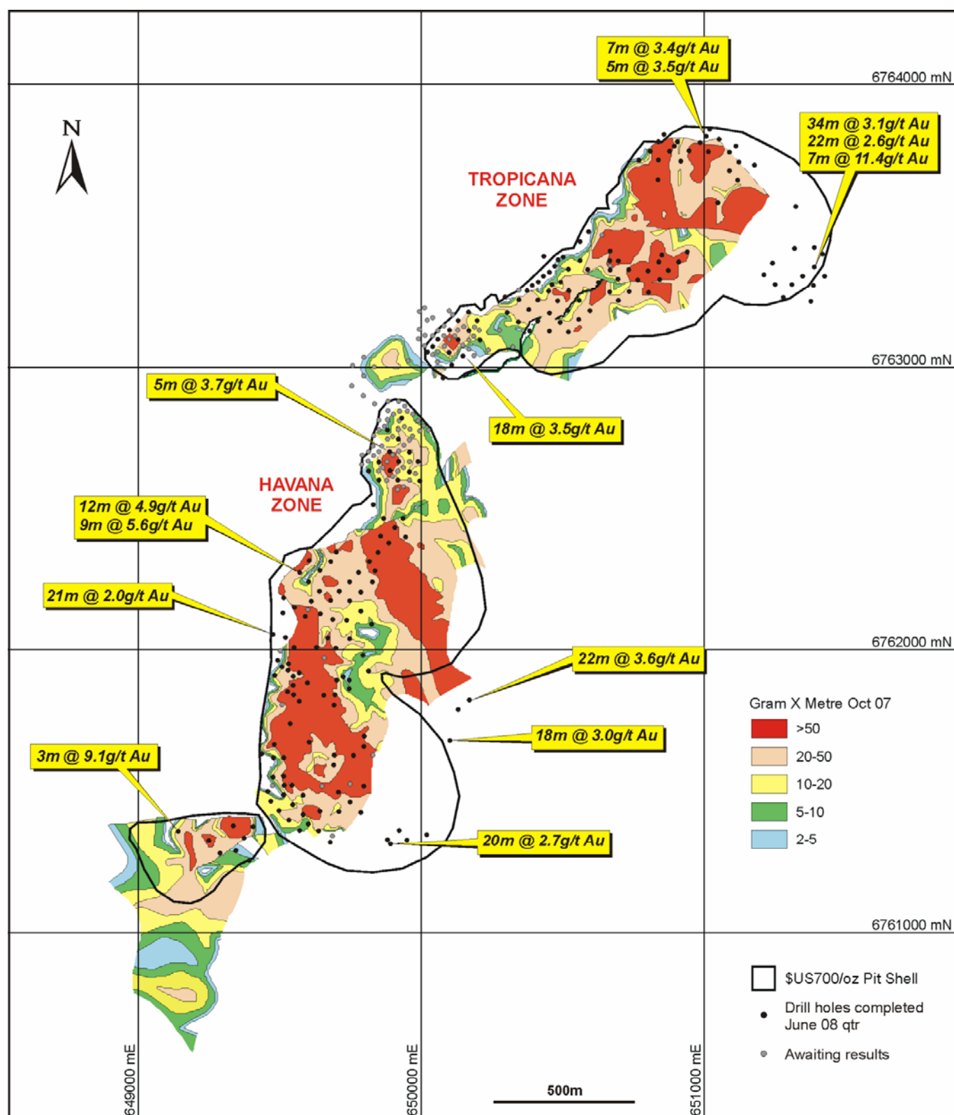
Figure 7: Tropicana JV – Prospect Plan Showing Significant Intercepts Outside November 2007 Resource Outline, g/t Au x Thickness Contours and Location of Havana and Tropicana Open Pit Resource Outlines
