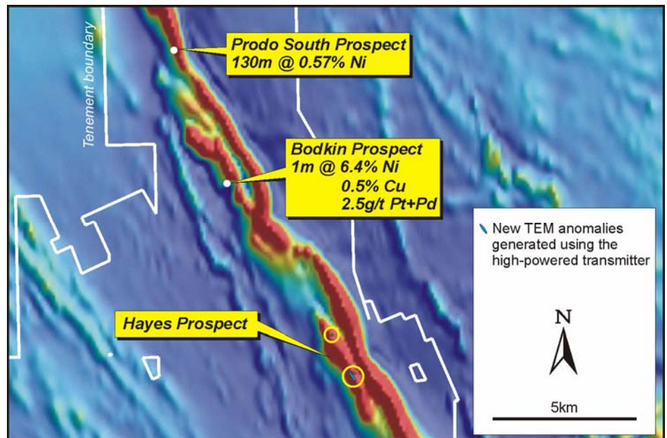
Figure 13: Wiluna JV – Prodo South, Bodkin and Hayes Prospect Locations, Significant Drill Results and New Hayes TEM Anomalies Over Aeromagnetics
