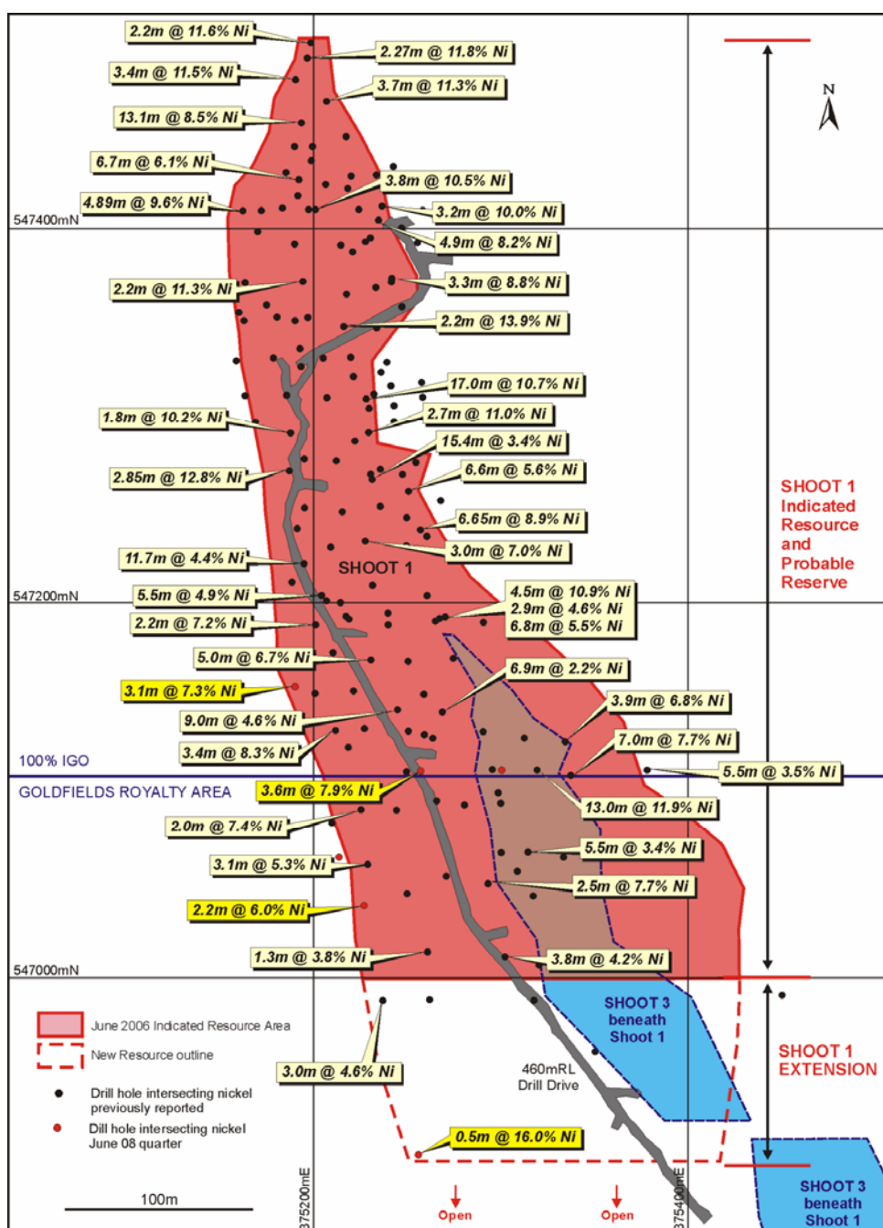
Figure 3: McLeay – Shoot 1 Plan Showing 460 Drill Drive, Significant Intercepts and Shoot 1 Outline
