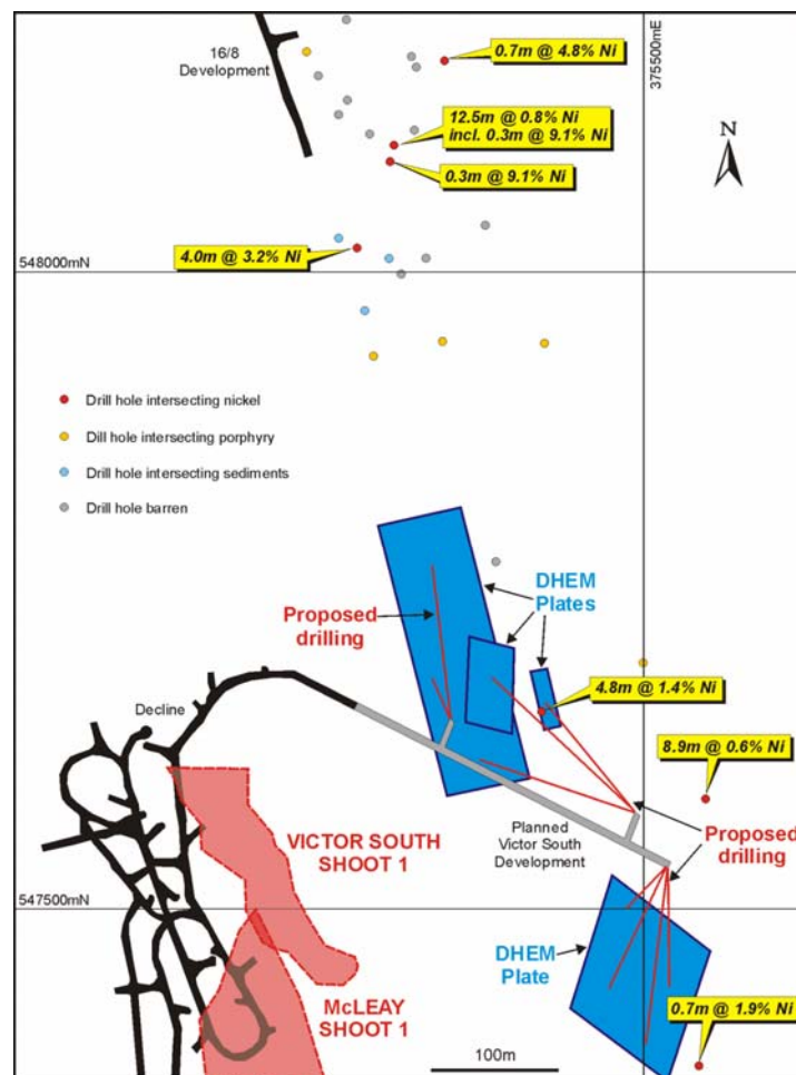
Figure 5: Plan Showing the Locations of Long South High Conductance TEM Plates and Proposed Drill Drive and Drill Holes in Relation to the 16-8 Long South Drill Drive, Victor South and McLeay Ore Bodies
