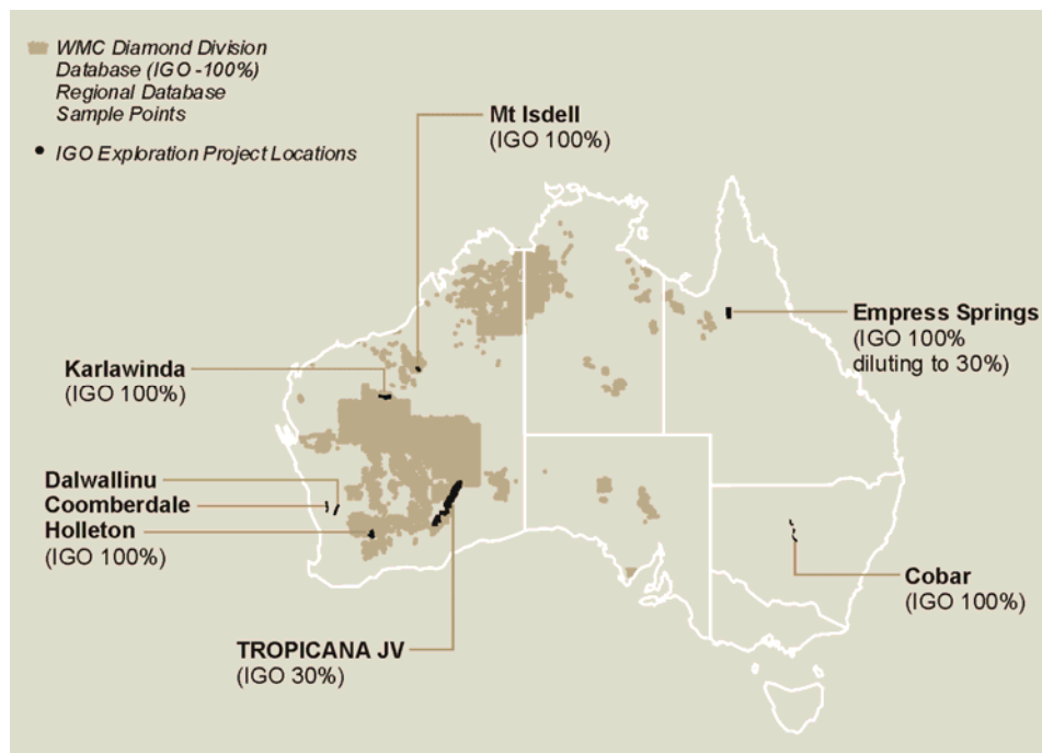
Figure 6: IGO Gold and Non-Nickel Base Metal Project Locations
