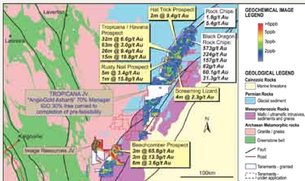
Figure 7: Tropicana JV - Tenure, Gold Geochemical Anomalies, Significant Drill Intercepts and Rock Chips Over the Yilgarn Craton - Fraser Range Mobile Belt Collision Zone
