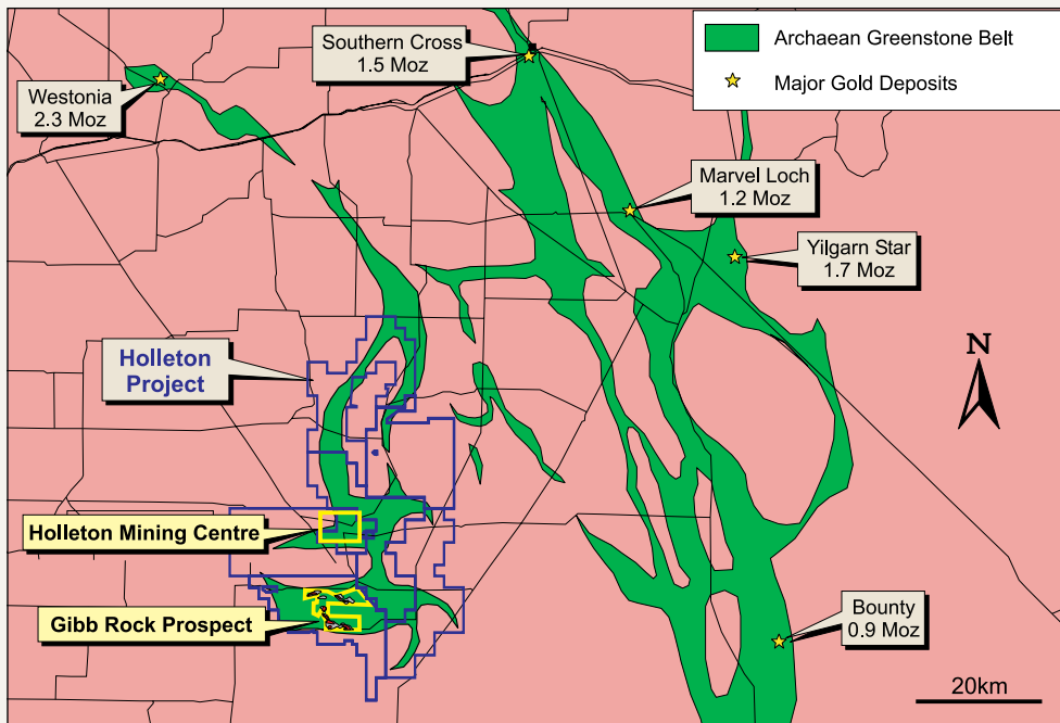
Figure 10: Holleton Project - Tenure Over Regional Geology Showing Prospect Locations and Large Gold Mines in District
