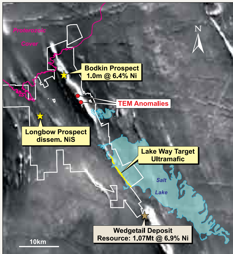
Figure 16: Wiluna JV - Tenure, Prospects and Significant Intercepts Over Aeromagnetic Image
