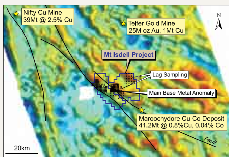
Figure 18: Mt Isdell JV - Tenure and Significant Nearby Mines Over Gravity Image
