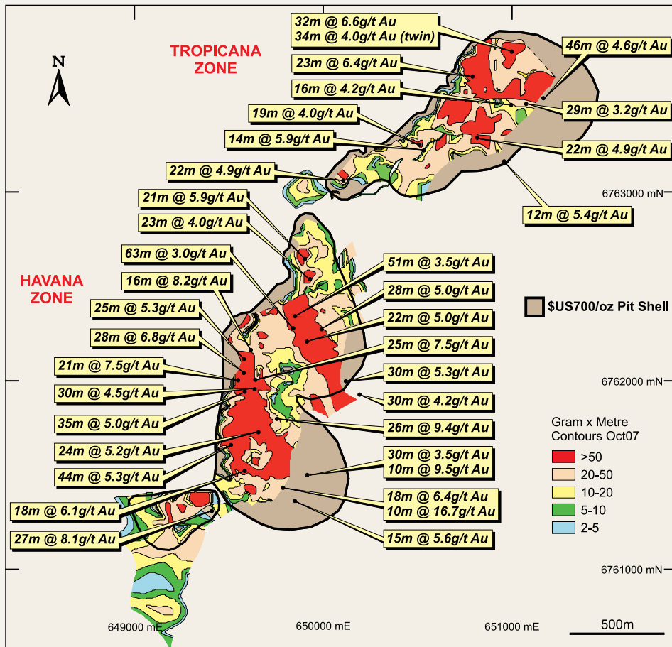
Figure 8: Tropicana JV - Tropicana/Havana December 2007 Conceptual Open Pit Outlines, Significant Intercept Locations and October 2007 g/t Au x Thickness (m) Contours
