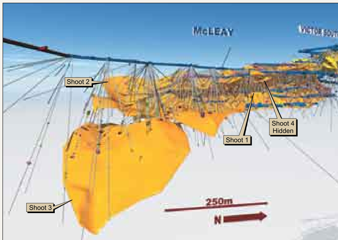
Figure 3: McLeay Deposit - 3D Isometric Model Showing Nickel Shoots, Drill Holes and Development
