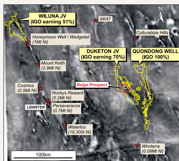
Figure 14: North-Eastern Goldfields Nickel Project Locations and Selected Nickel Mines Over Aeromagnetic Image
