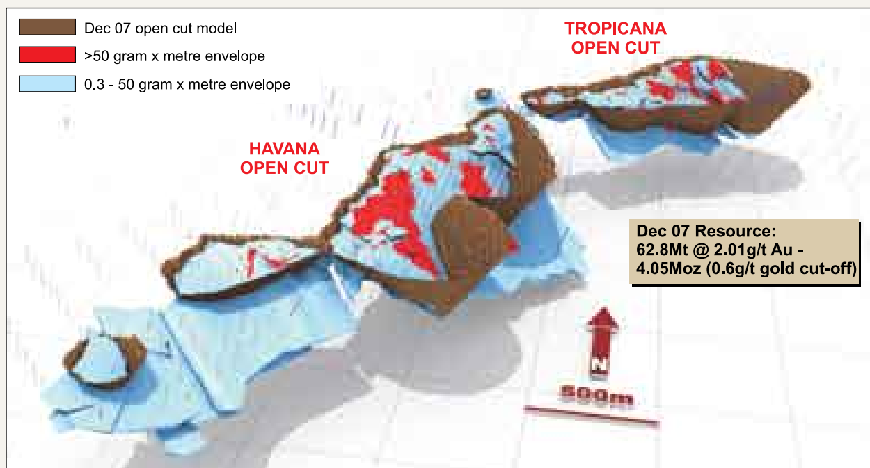
Figure 9: Tropicana JV - Isometric Model Showing 0.3 g/t Au Mineralised Envelope, > 50 gram Au x Metre Envelope and December 2007 Preliminary Conceptual Open Pit Outlines
