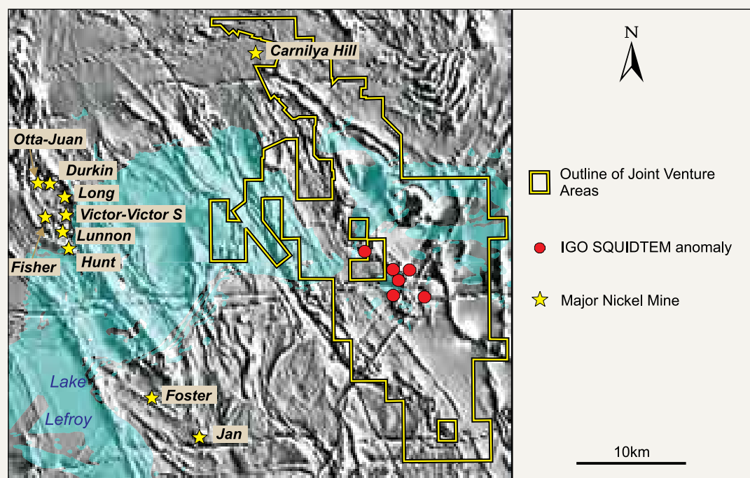
Figure 17: Lake Lefroy JV's - Tenure, Lake Coverage and Major Nickel Mines Over Aeromagnetic Image
