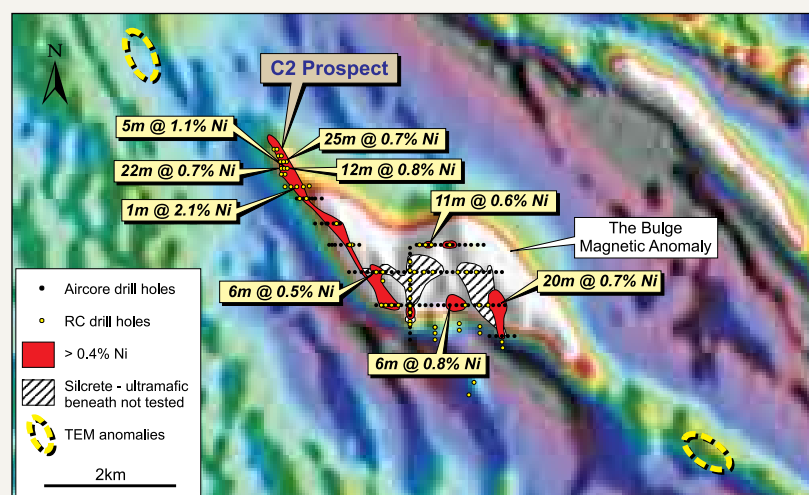
Figure 15: Duketon JV - Bulge Prospect Significant RC and AC Drill Results, >0.4% Ni Anomalism and TEM Anomalies Over Aeromagnetic Image
