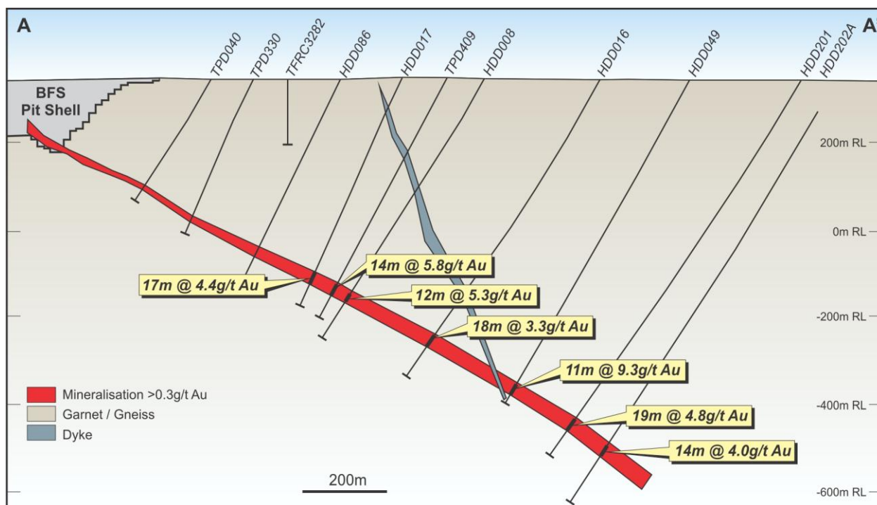
Figure 7: Tropicana JV – Havana Deeps TPD040 – HDD202A cross section showing continuation of gold mineralised zone down plunge from the base of the proposed Havana open pit.
