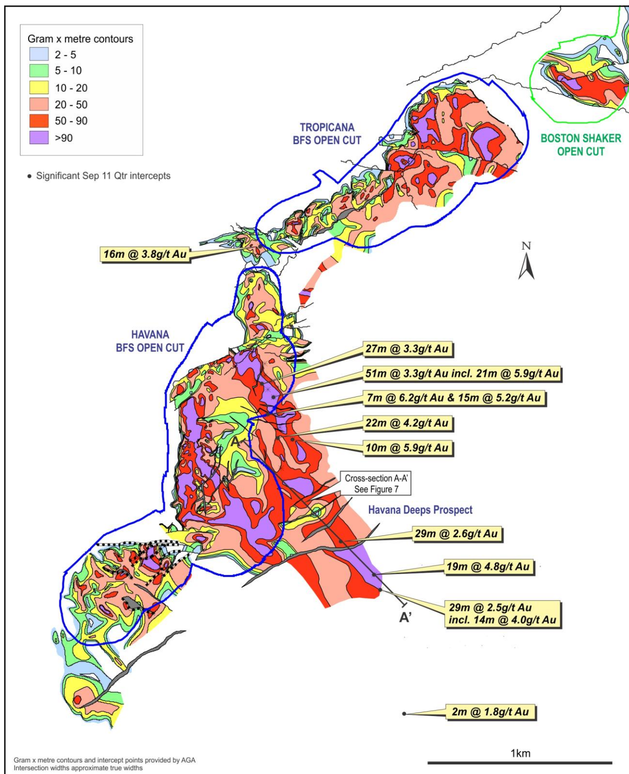
Figure 6: Tropicana JV – Proposed Boston Shaker, Tropicana, Havana and Havana South Open Pit Outlines, g/t Au x Thickness (m) Contours in 3D Isometric Model and significant September 2011 quarter intercepts.
