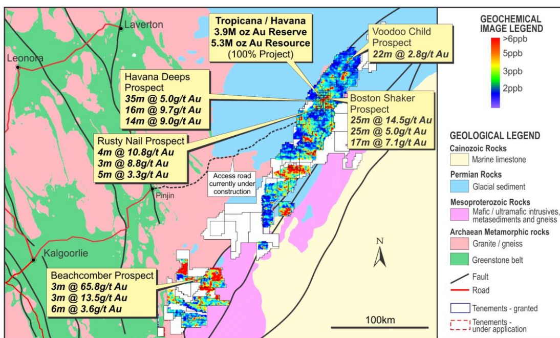
Figure 5: Tropicana JV – Tenure, Tropicana and Havana Reserve Locations, Gold Geochemical Anomalies, Significant Drill Intercepts and Selected Prospect Locations
