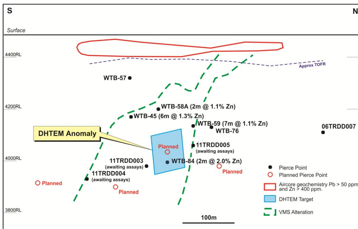
Figure 4: Jaguar / Bentley Operation – Lagonda Prospect Longitudinal Projection showing significant intercepts, planned drilling, down hole TEM anomaly and sericite hydrothermal alteration zone.
