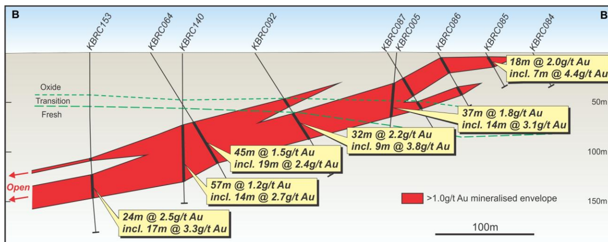
Figure 10: Karlawinda Project – Bibra long section of central gold shoot (refer Figure 9 for location)
