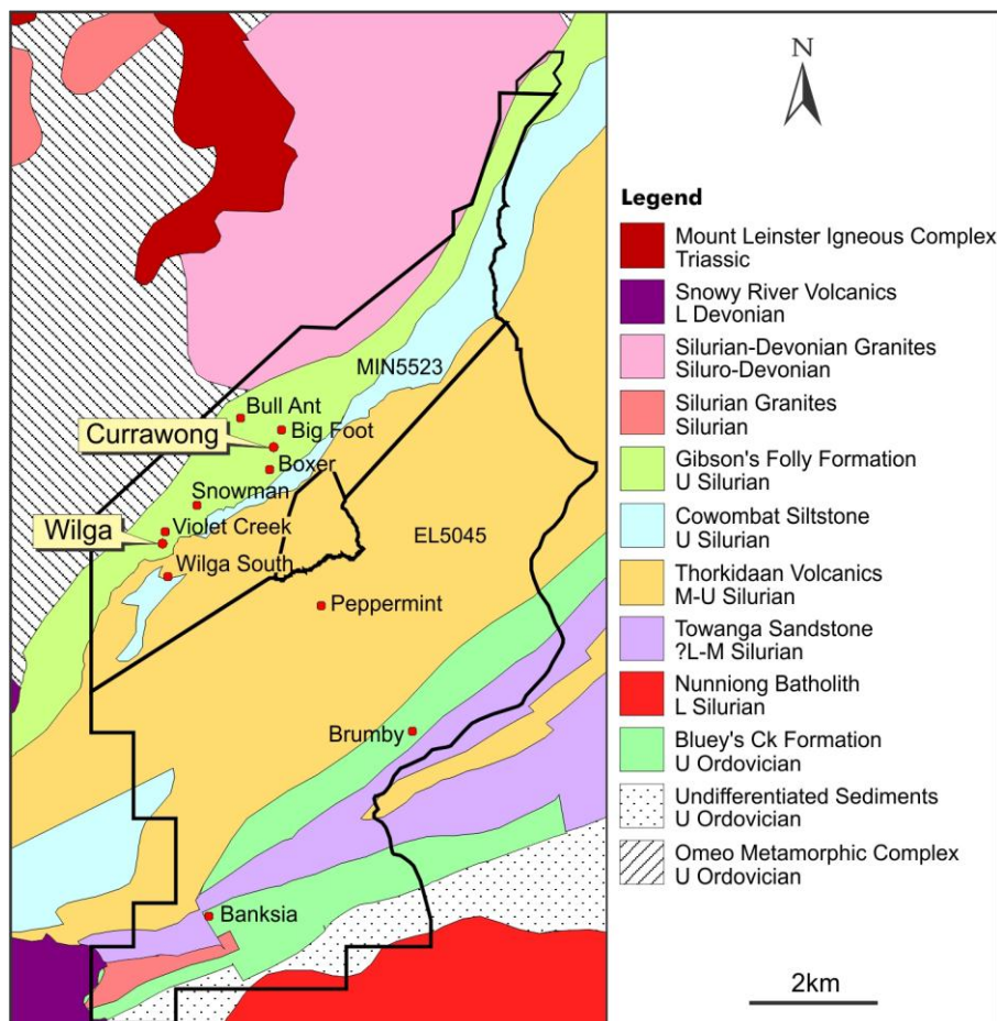
Figure 8: Stockman Project – Regional Geology, Tenure, Deposits and Prospects
