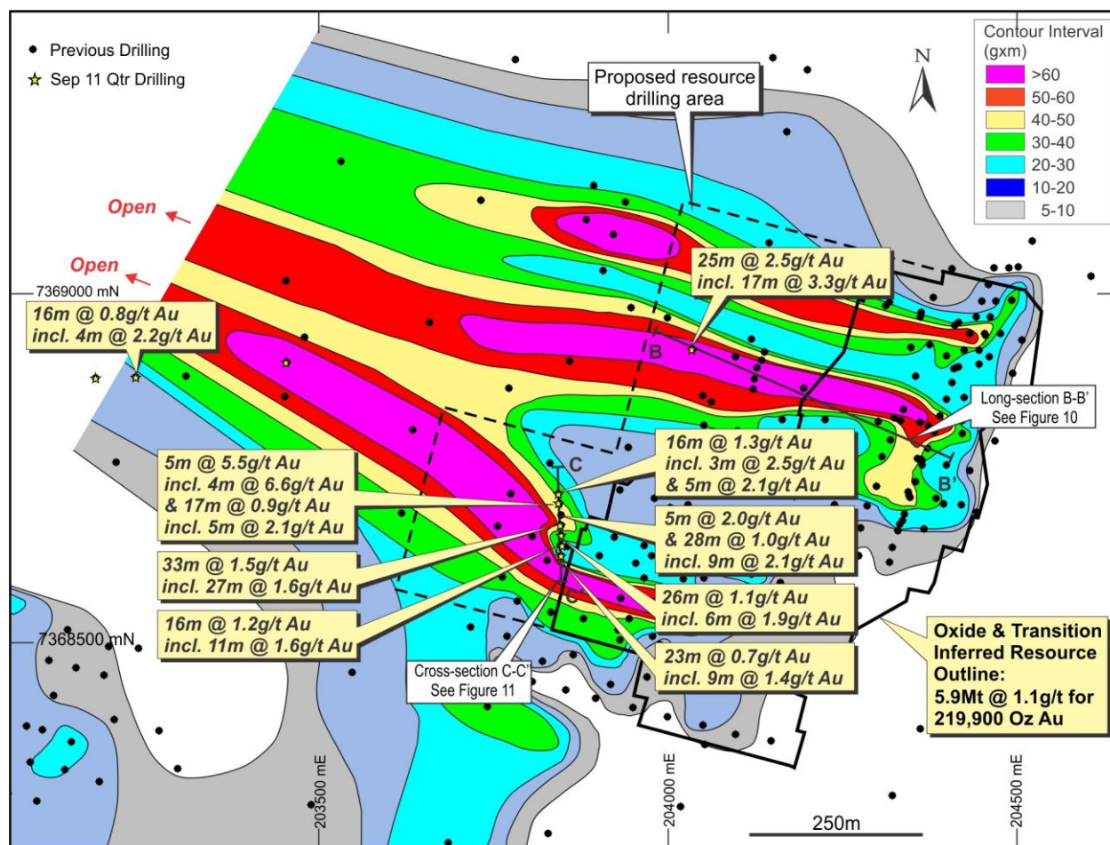
Figure 9: Karlawinda Project – Bibra Prospect Drill Defined Gold Anomalies, Significant September 2011 quarter drill Intercepts, Figures 10 and 11 Cross section location over g/t Au x metre contours.
