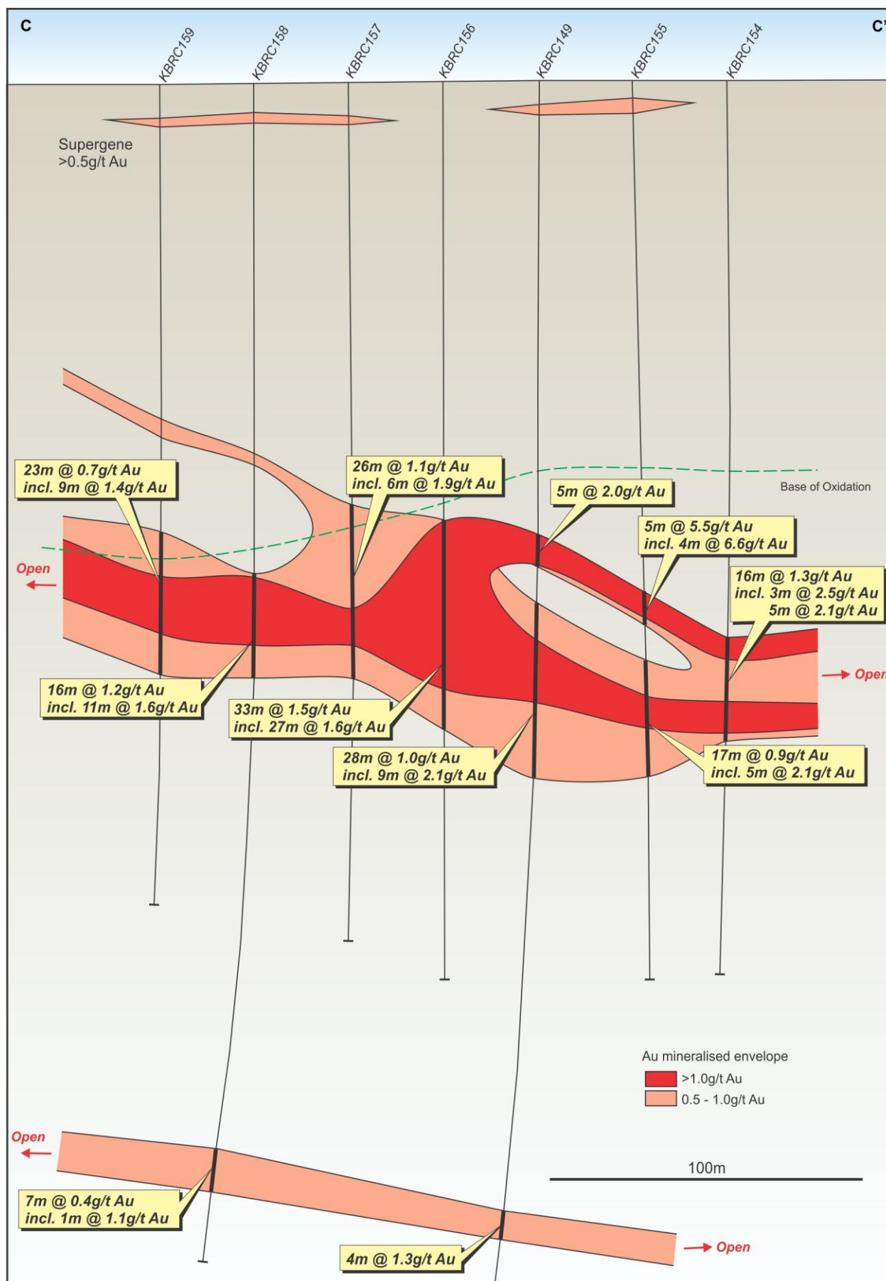
Figure 11: Karlawinda Project – Bibra cross-section of southern gold shoot (Refer Figure 9 for location)
