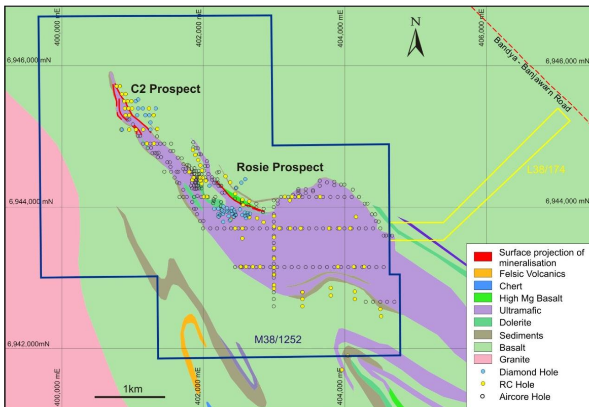
Figure 2: Location of the Rosie deposit within Mining Lease M38/1252 over interpreted geology, with current drill hole locations.
