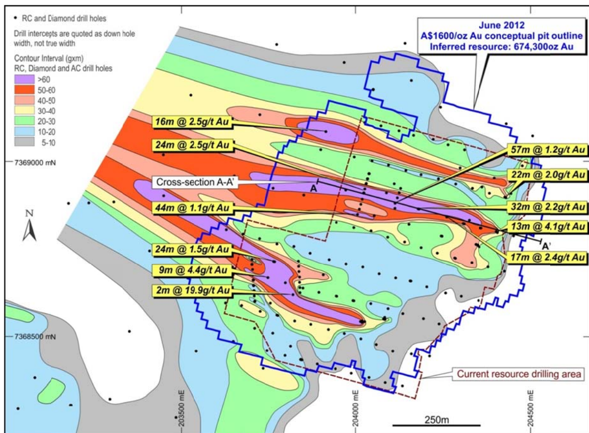
Figure 2: Bibra Resource area – gram x metre contours with A$1,600/oz Au June 2012 conceptual optimised pit outline, RC and diamond drilling collar locations (AC collars omitted) and Figure 3 A-A' cross-section location.
