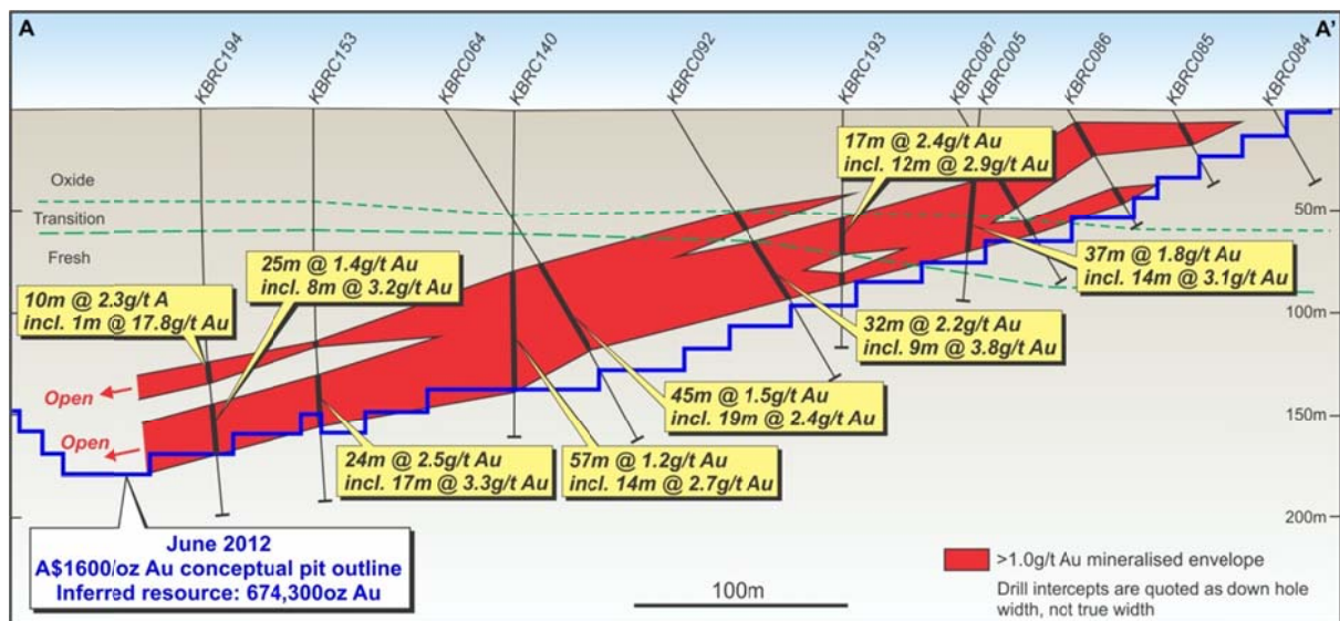
Figure 3: Bibra cross-section with mineralisation and June 2012 conceptual optimal pit outline ($1,600/oz Au).
