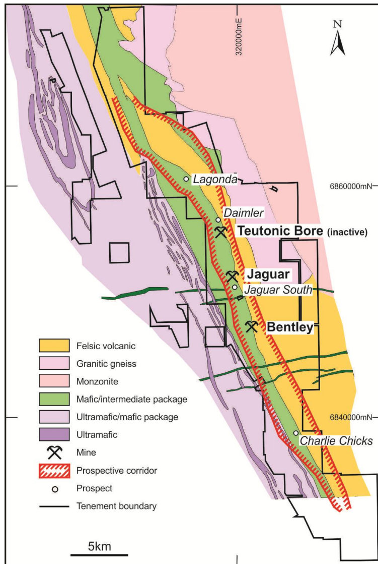
Figure 1: Jaguar and Bentley Operations regional geology and prospective mine corridor.
