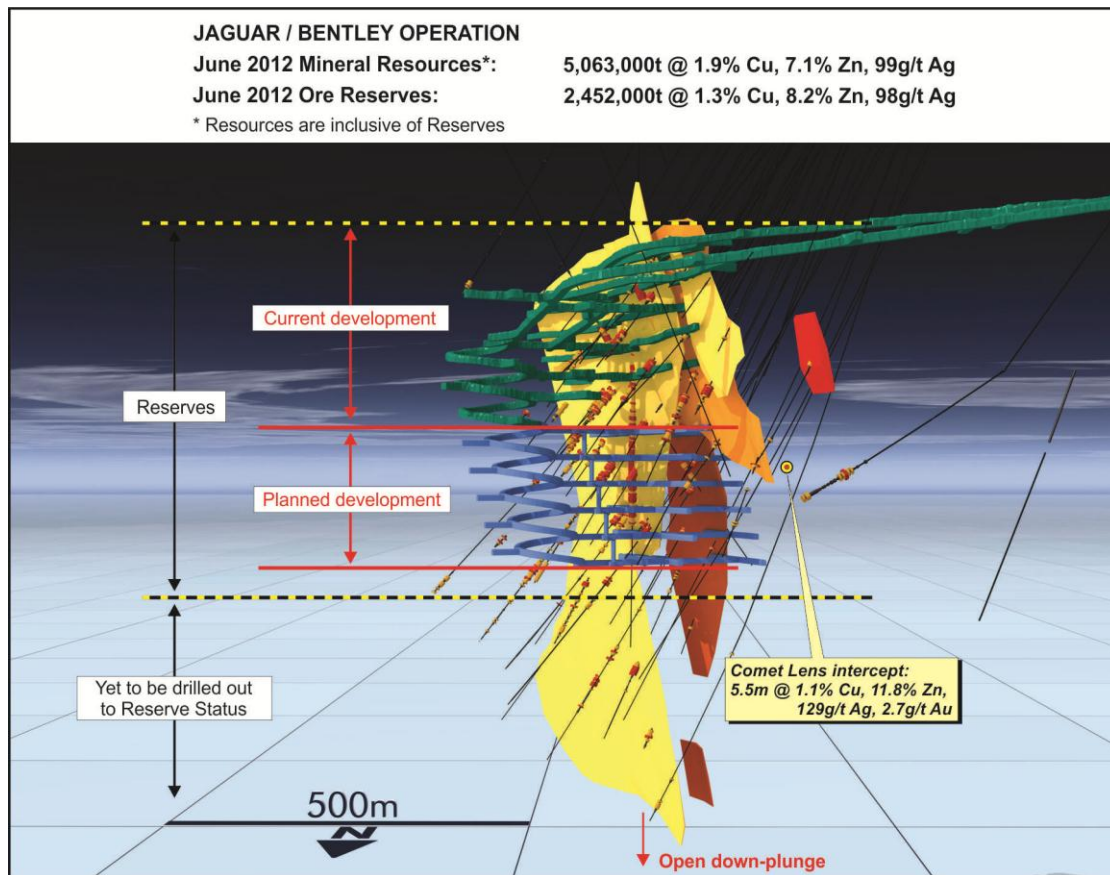
Figure 2: Jaguar/Bentley Operation Resource and Reserves showing Bentley deposit and Comet Lens intercept.
