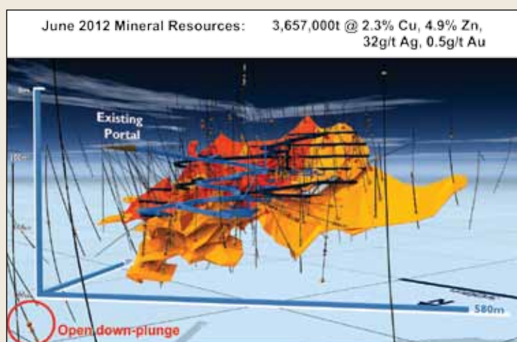
Figure 12: Stockman Cu-Zn-Ag-Au Project: Wilga Deposit - 3D isometric projection showing mineralised envelopes, drilling, planned development and down plunge mineralised intersections.
