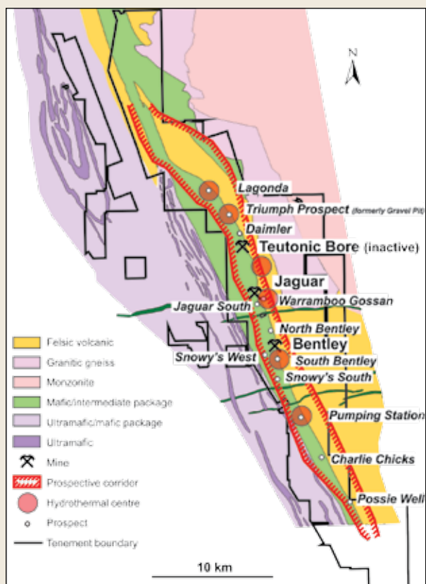
Figure 4: Jaguar/Bentley Cu-Zn-Ag Operation - Tenure, regional geology, mines and significant prospect locations.
