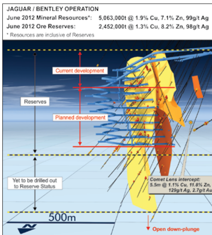
Figure 5: Jaguar/Bentley Cu-Zn-Ag Operation - Bentley Mine - 3D isometric projection showing mineralised envelopes, drilling and planned development.
