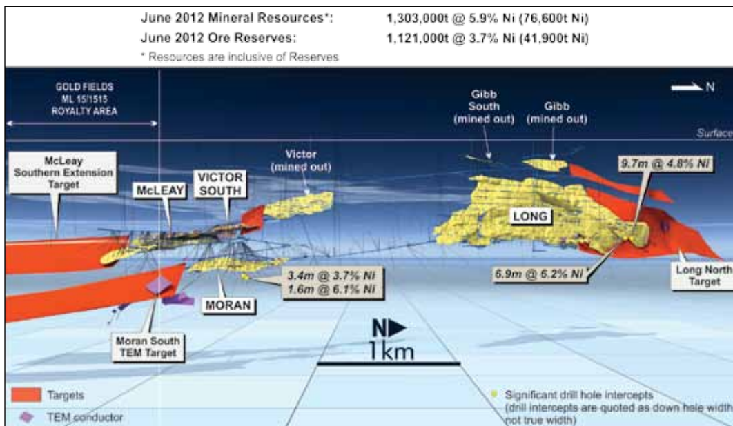
Figure 3: Long Nickel Operation - Longitudinal Projection showing target areas, TEM conductors and significant FY2012 intercepts.
