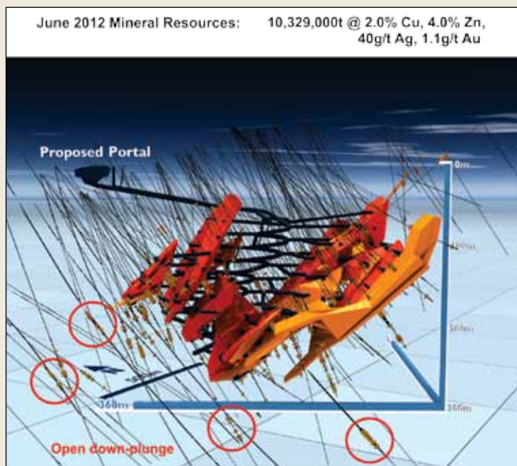
Figure 11: Stockman Cu-Zn-Ag-Au Project: Currawong Deposit - 3D isometric projection showing mineralised envelopes, drilling, planned development and down plunge mineralised intersections.
