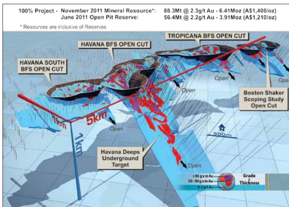
Figure 9: Tropicana JV - Proposed Boston Shaker, Tropicana, Havana and Havana South open pit outlines, g/t Au x thickness (m) contours in 3D isometric model.
