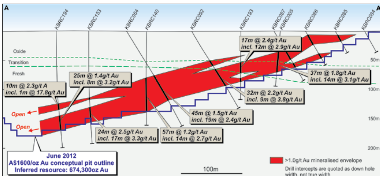
Figure 15: Karlawinda-Bibra Prospect Long-section showing oxide, transition and fresh mineralised zones.
