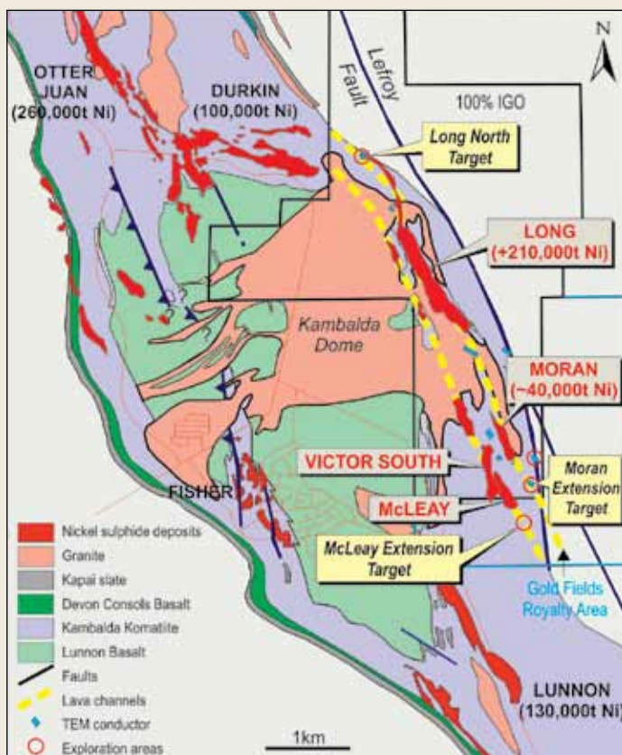
Figure 2: Long Nickel Operation - Regional geology, tenure, nickel shoots and targets.
