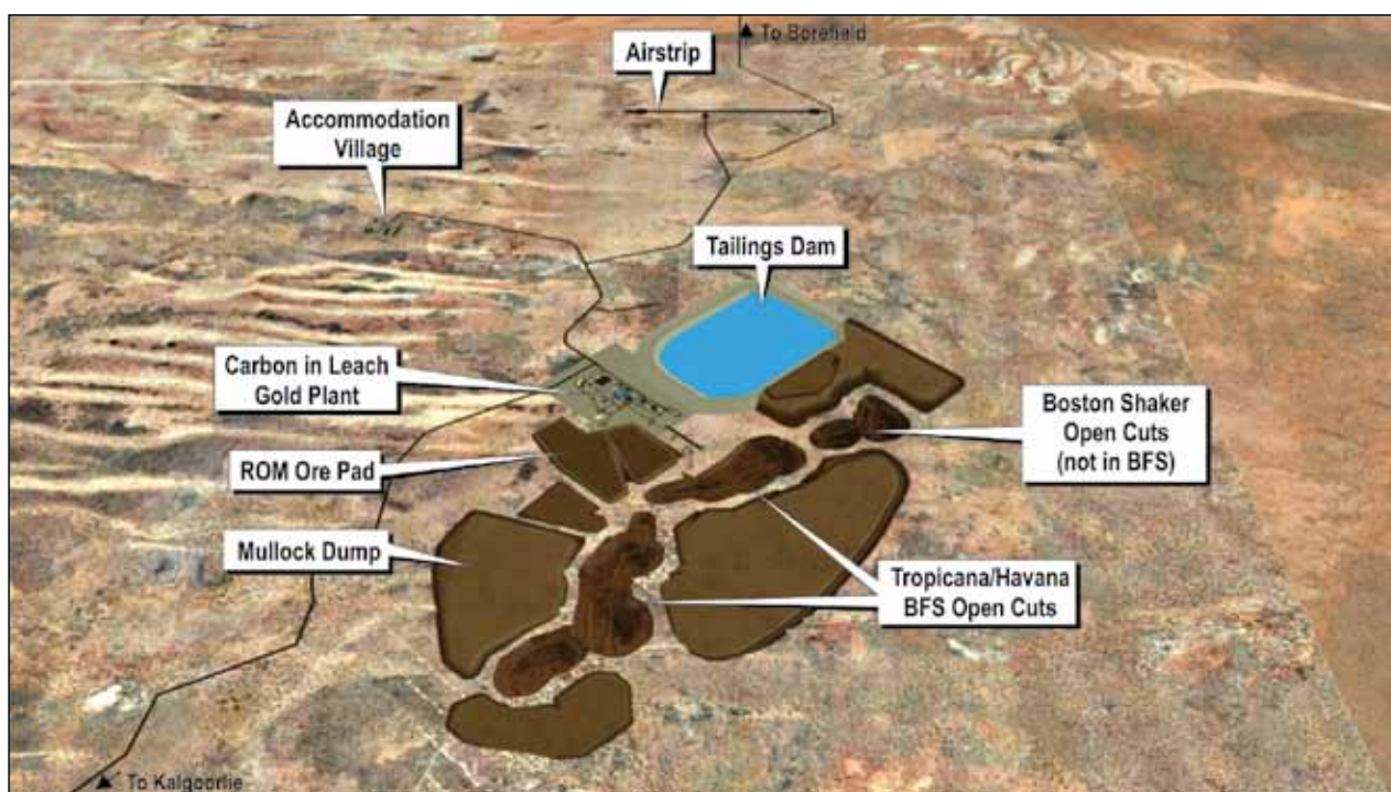
Figure 7: Tropicana JV - Computer generated model showing the layout of proposed Tropicana, Havana and Boston Shaker open cuts, mullock dumps, gold plant, tailings dam, airstrip and accommodation village.
