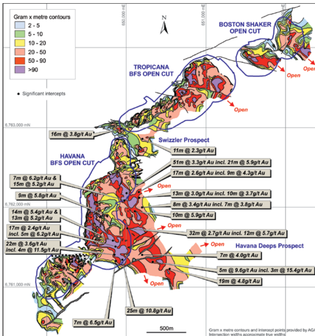
Figure 10: Tropicana JV - Proposed Boston Shaker, Tropicana, Havana and Havana South open pit outlines, significant FY2012 drill hole intercepts and g/t Au x thickness (m) contours.
