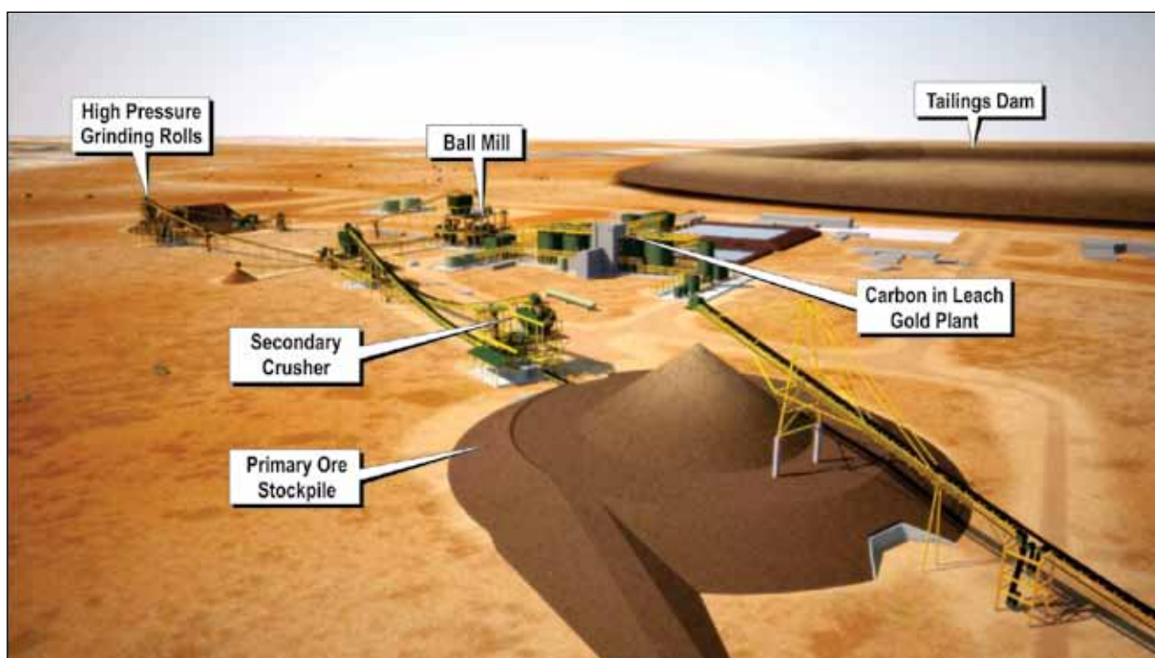
Figure 8: Tropicana JV - Computer generated model of proposed plant layout.
