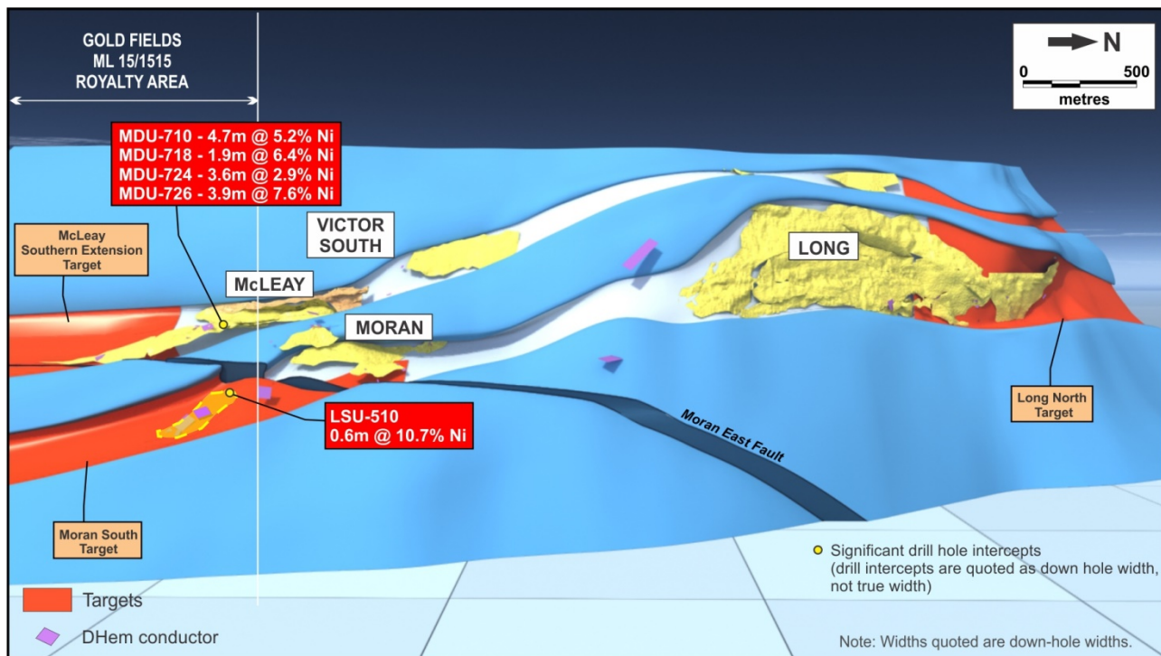
Figure 3: Long Operation – Longitudinal Projection showing Target areas, DHEM conductors
