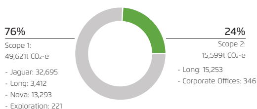
FIGURE 22 GREENHOUSE GAS EMISSIONS
