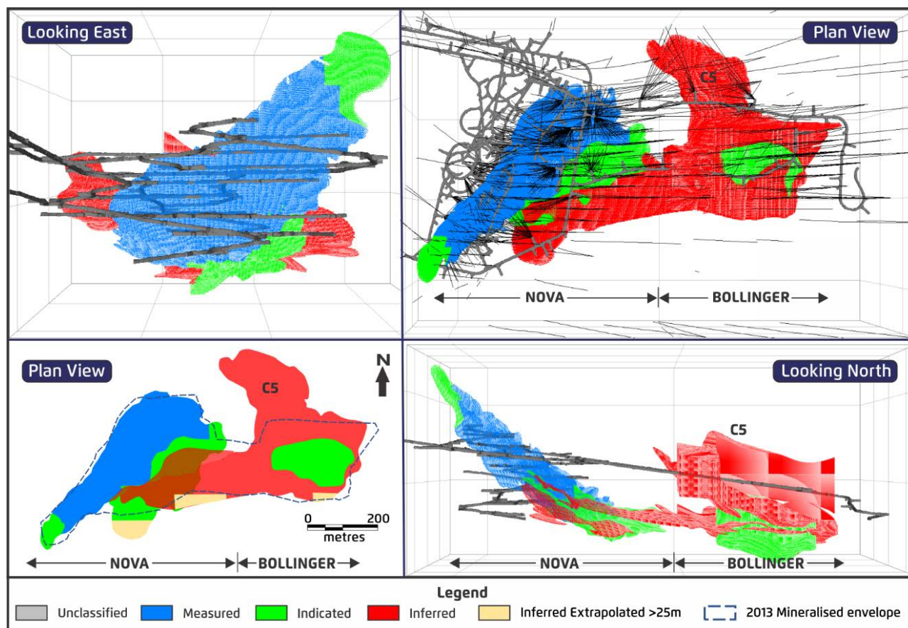
Figure 3: Various projections of the Nova-Bollinger deposits showing Mineral Resource Classification
