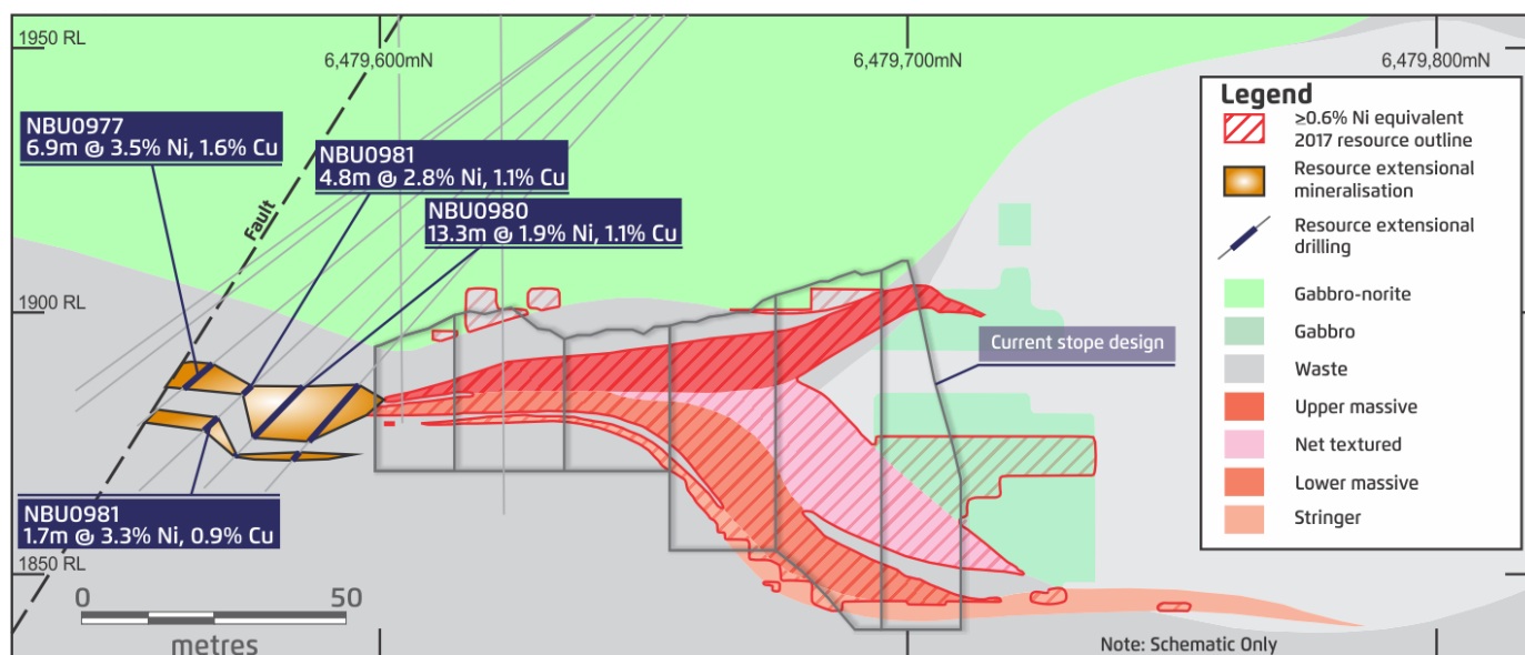
Figure 2: Example section from Bollinger (518900mE) looking west showing recent drill intersections returned outside the current Mineral Resource
