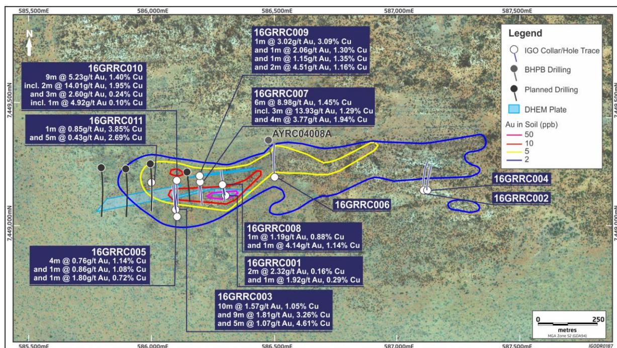
Figure 3: Grapple Prospect showing the location of the four planned drillholes, the eleven completed drill holes and the conductive plates to be tested.
