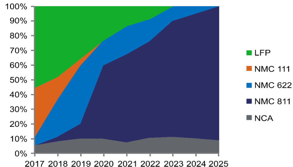
Increasing Nickel Content in Batteries (1)
