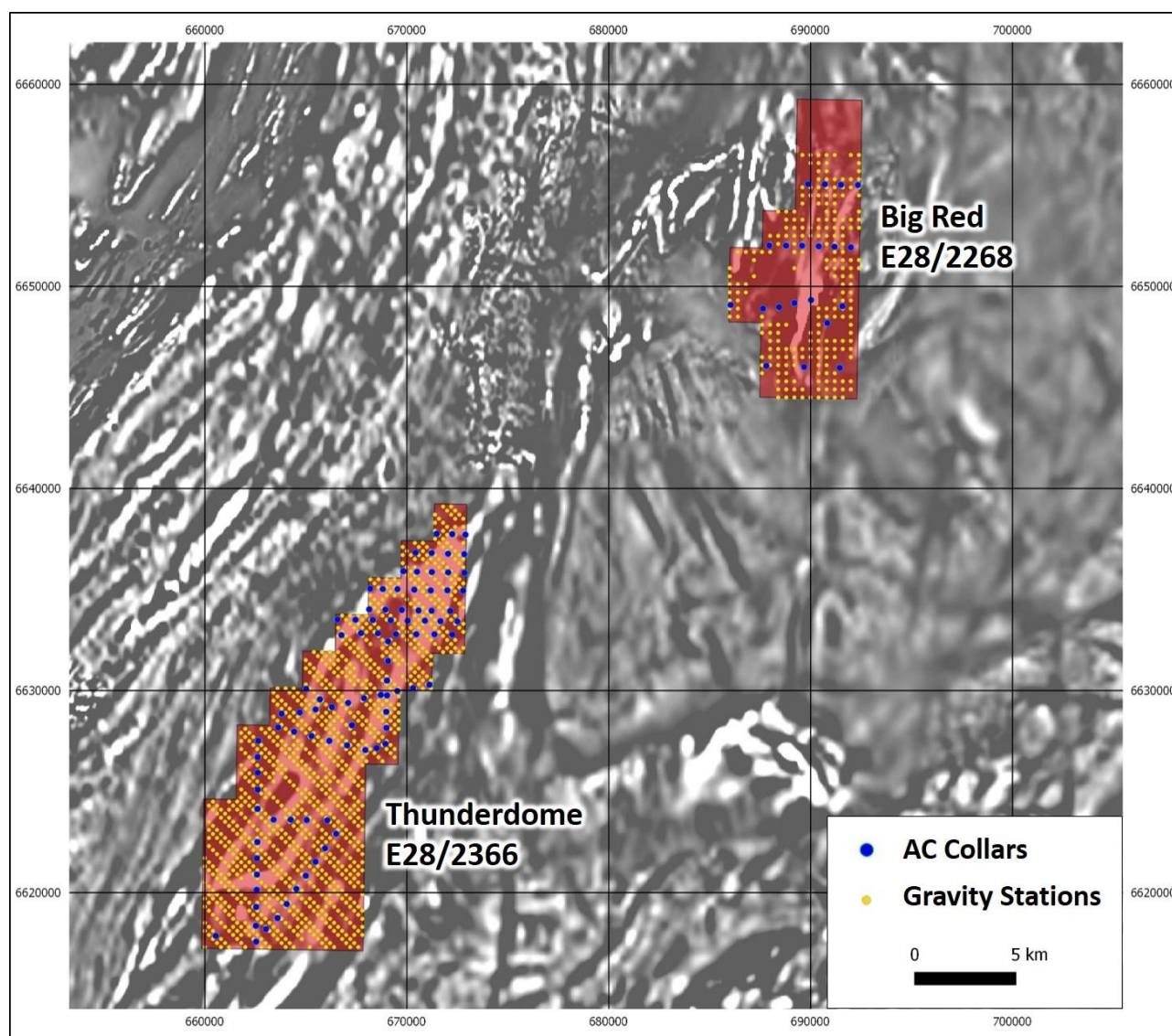
Image 2 Big Red and Thunderdome Tenements on greyscale TMI 1VD RTP regional aeromagnetics. Gravity stations and completed AC collars are shown
