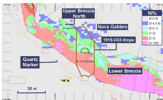
Example stope – section 6,479,755mN looking north
