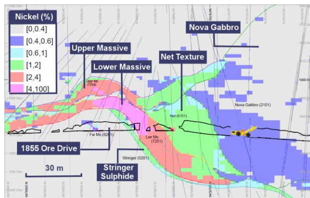
Bollinger cross section – looking West on 518,900mE
