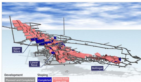
Nova-Bollinger life-of-mine development and stoping plan
