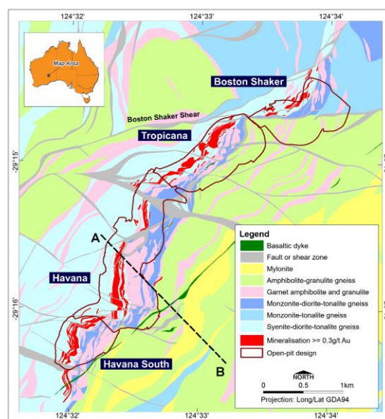
Geology plan of the Tropicana Gold Mine
