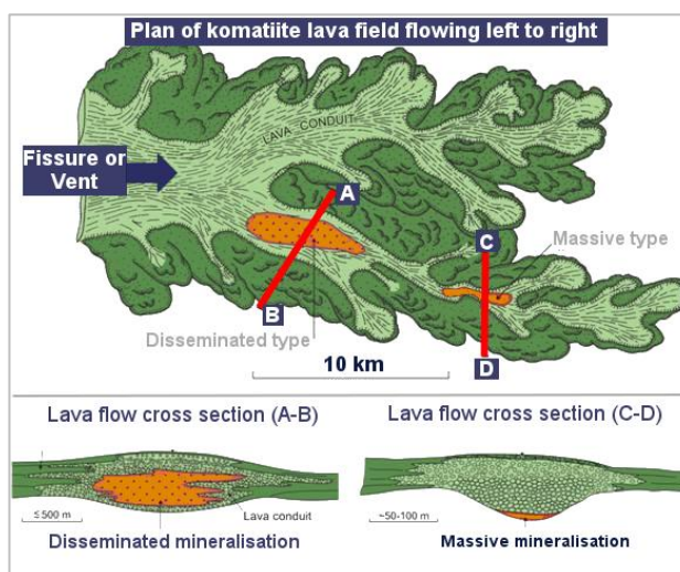
Lava-channel models for Kambalda-style nickel deposits
