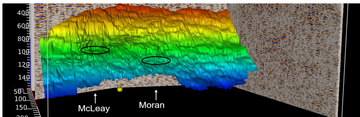
3D seismic survey interpretation of the ultramafic-basalt interface
