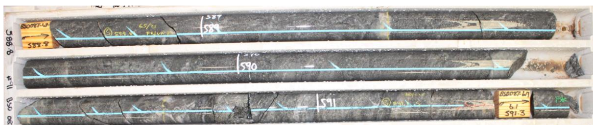
Example drill core from Tropicana resource definition drilling
