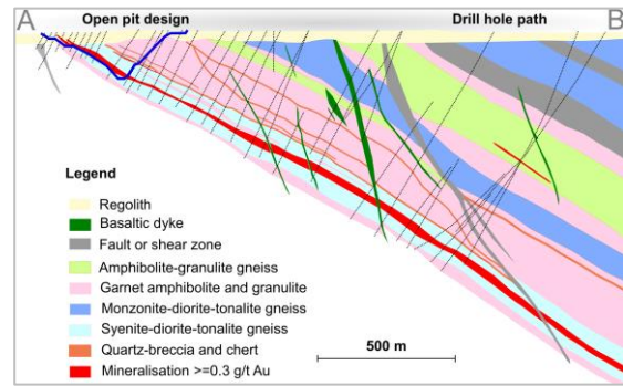
Havana Deposit geological cross section looking northeast
