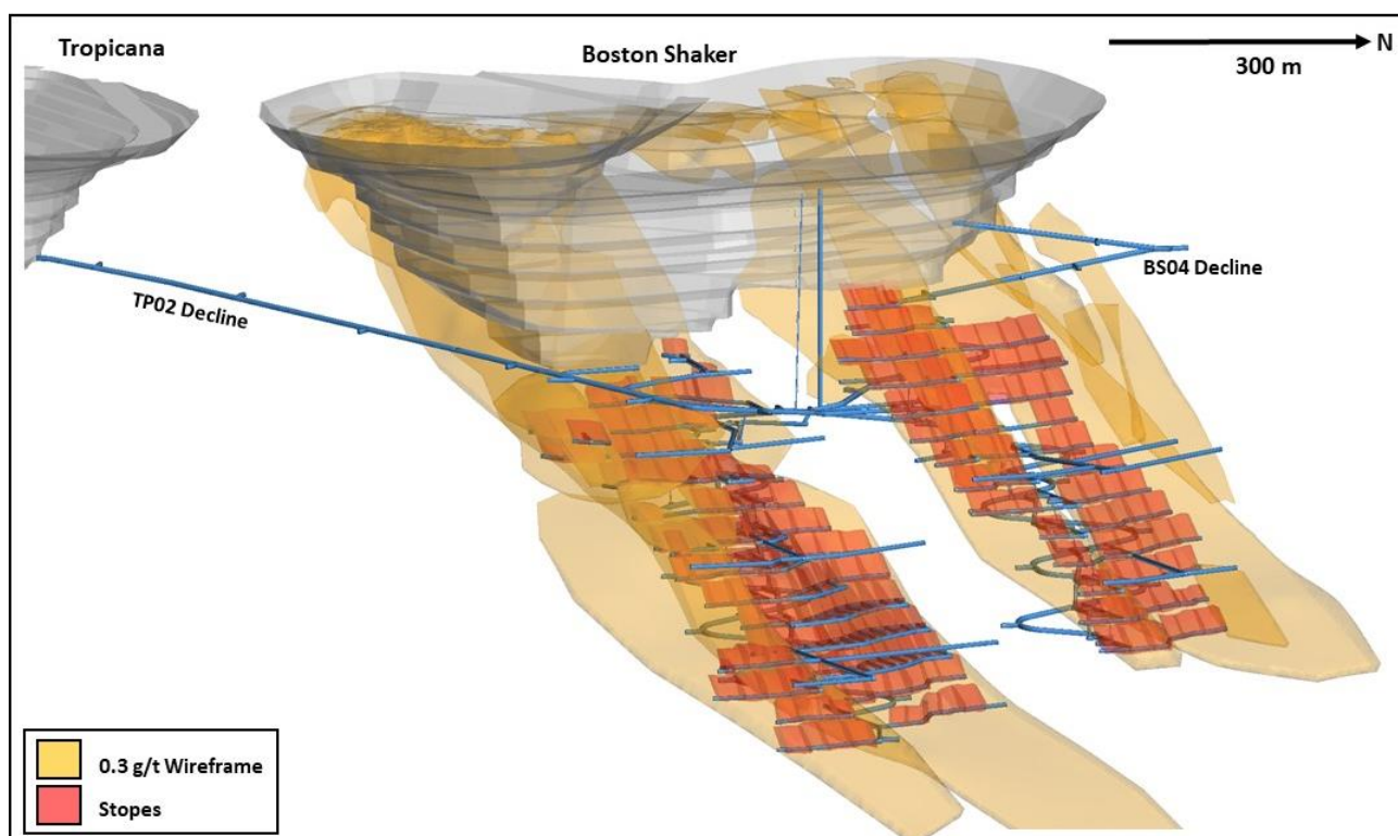
Figure 2: Boston Shaker Decline Location and Stope Design
