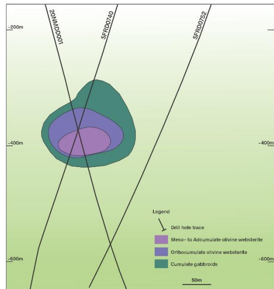
Cross section through the Orion chonolith
