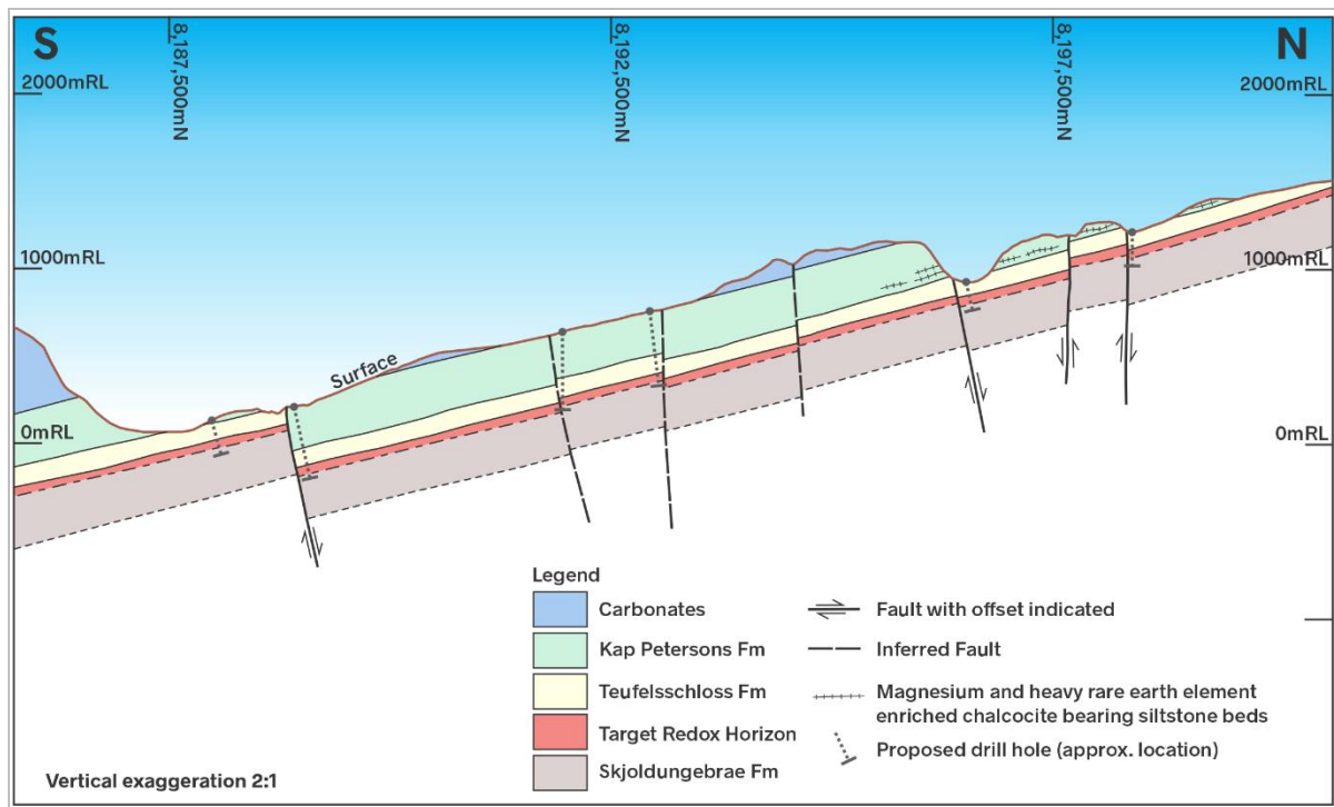
Schematic long section geological interpretation looking west between locations S to N on previous image
