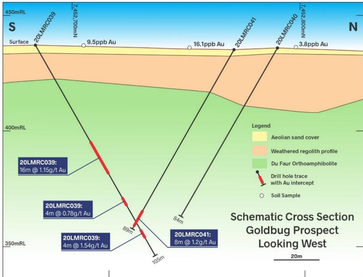
Schematic cross section of the Goldbug Prospect drilling, surface geochemistry and geology – looking west
