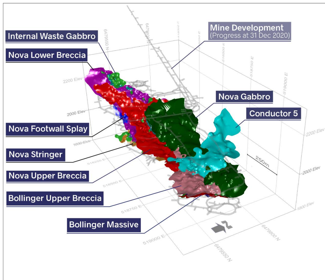
Selected estimation zones of the Nova-Bollinger CY20 MRE model
