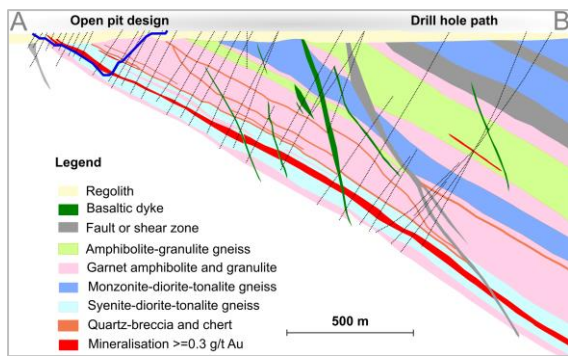
Havana Deposit northeast looking A—B section
