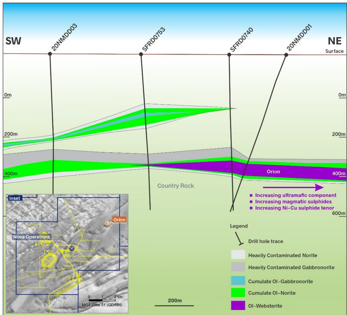
Schematic long section through the Orion Chonolith
