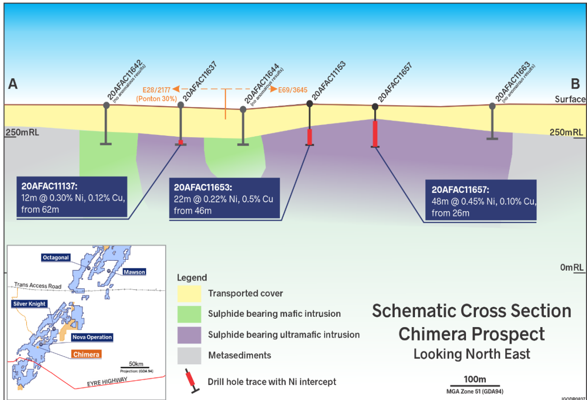
Chimera Prospect, schematic cross section looking northeast, interpreted geology and significant intersections
