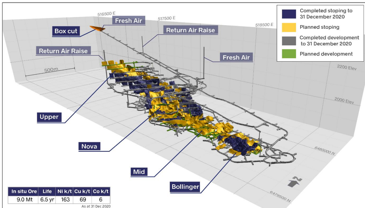
Nova CY20 completed stopes and mine development and future stopes
