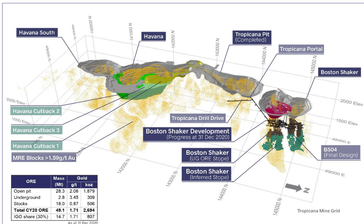
Tropicana ORE locations, mine development and mine plans
