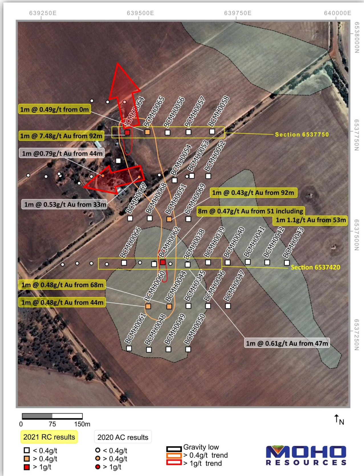
Figure 1: Location of recent RC drilling showing mineralisation >0.4 g/t Au and relationship between mineralised trends and gravity lows
