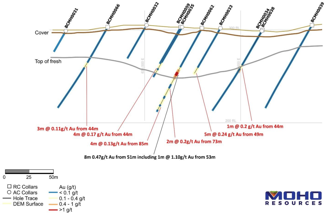
Figure 2: Section 6537420N showing Au mineralisation intersected in RC drilling
