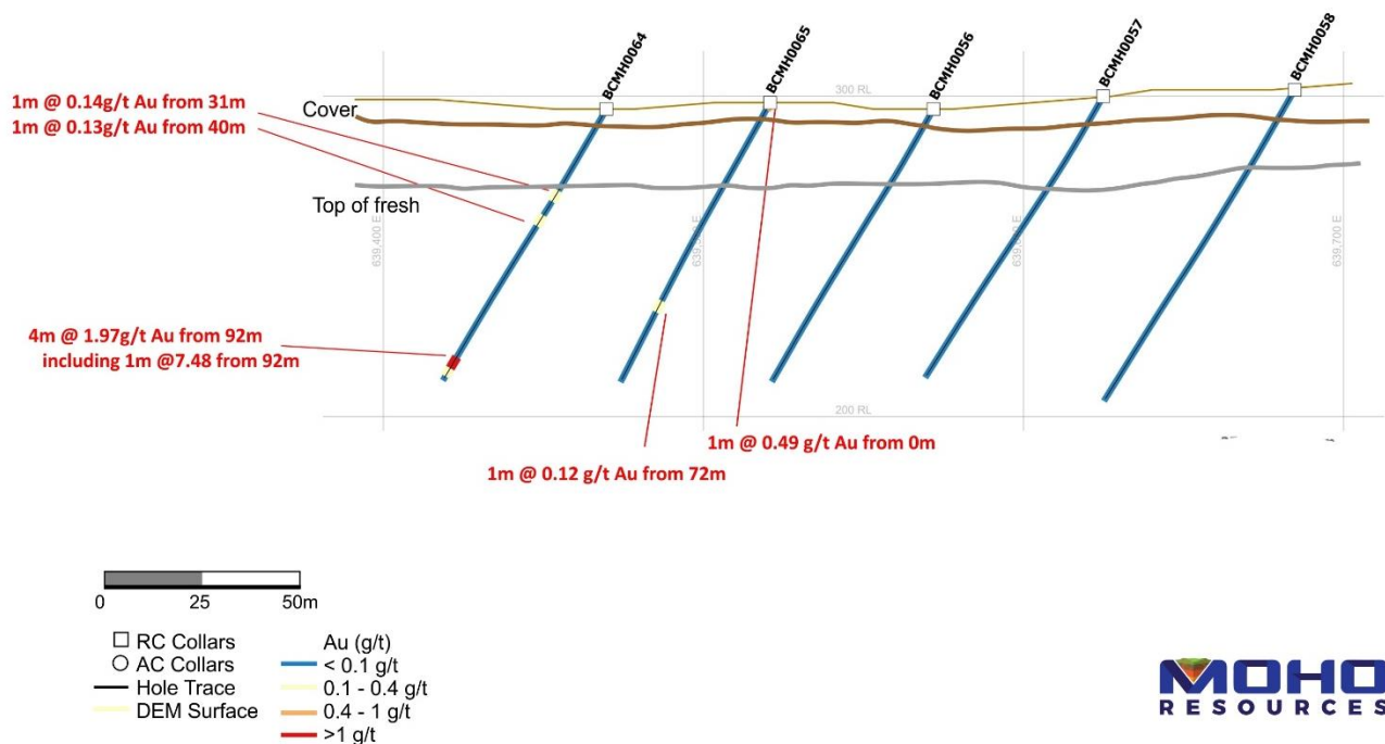
Figure 3: Section 6537750N showing Au mineralisation intersected in RC drilling
